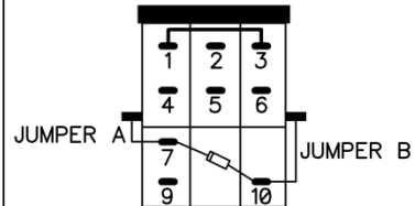
REAR VIEW CONNECTION LUGS
