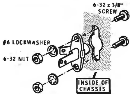
Detail 7C
