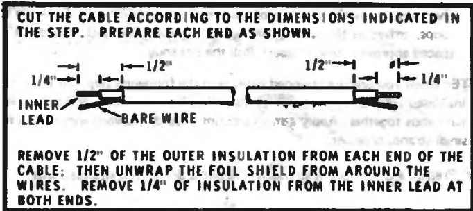
Detail 6A
