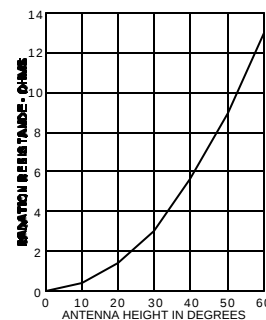
Fig. 50 — Same as Fig. 49, for heights below 60 degrees.
