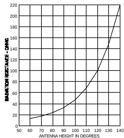
Fig. 49 — Radiation resistance vs. free space antenna height in electrical degrees for a vertical antenna over perfectly conducting ground, or over a highly conducting ground plane. This curve also may be used for center-fed antennas (in free space) by multiplying the radiation resistance by two; the height in this case is half the actual antenna length.
