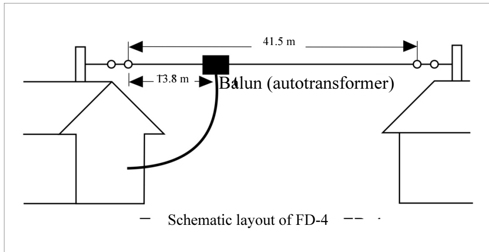
Coaxial fed Windom multiband antenna FD-4 fed
