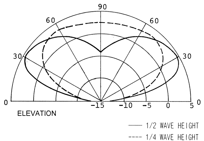
Figure 3. Radiation Patterns.
