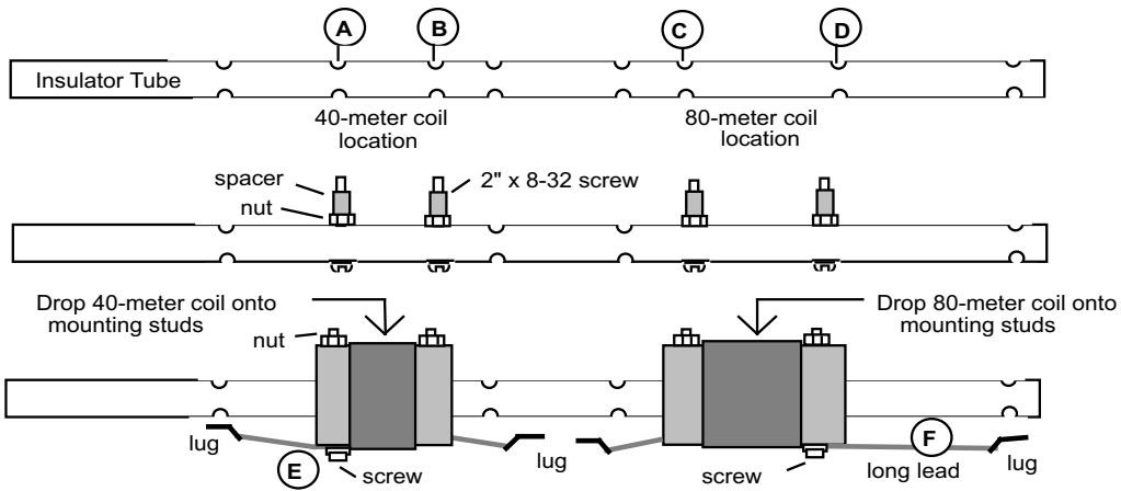
Figure-5: Loading Coil Mounting
