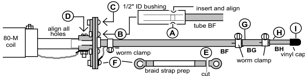
Figure-7: Upper Resonator ( 80-meter) Assembly
