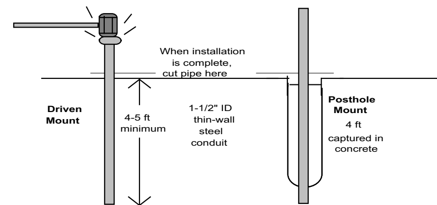
Figure-11A: Suggested base supports.
