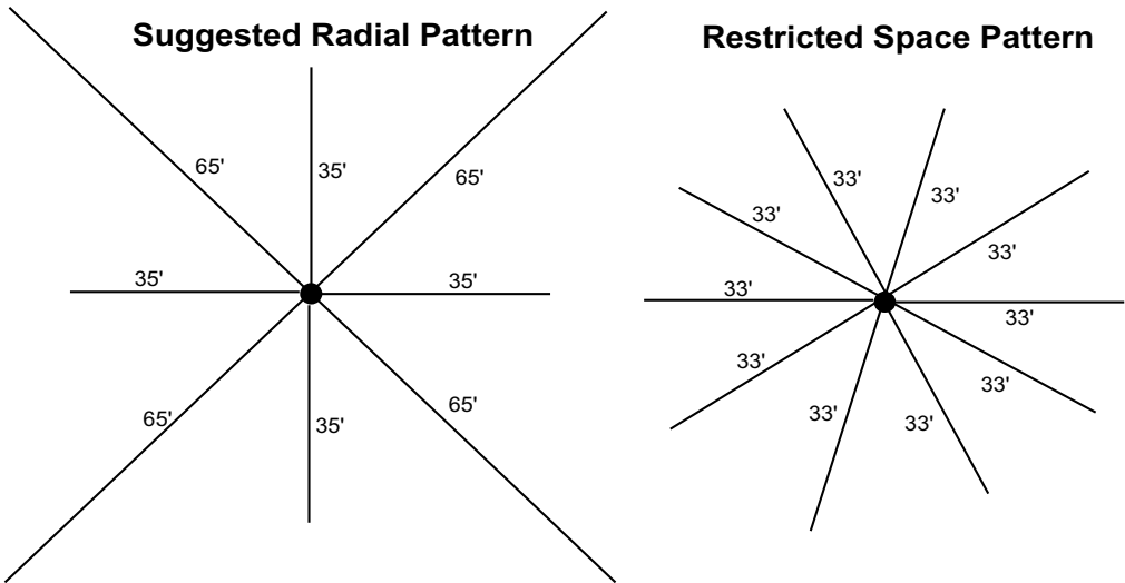
Figure-12B: Recommended radial-wire layout
