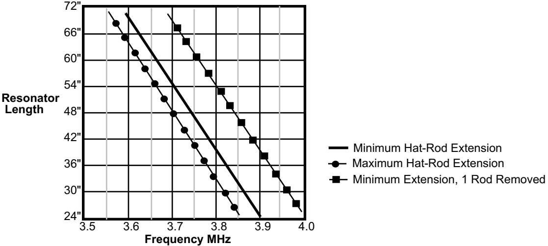
Graph-1: Suggested 80-meter Resonator Settings
