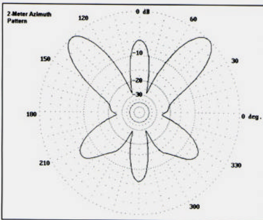
Fig. 4- Free-space azimuth pattern of the D2T at about 2 meters.
