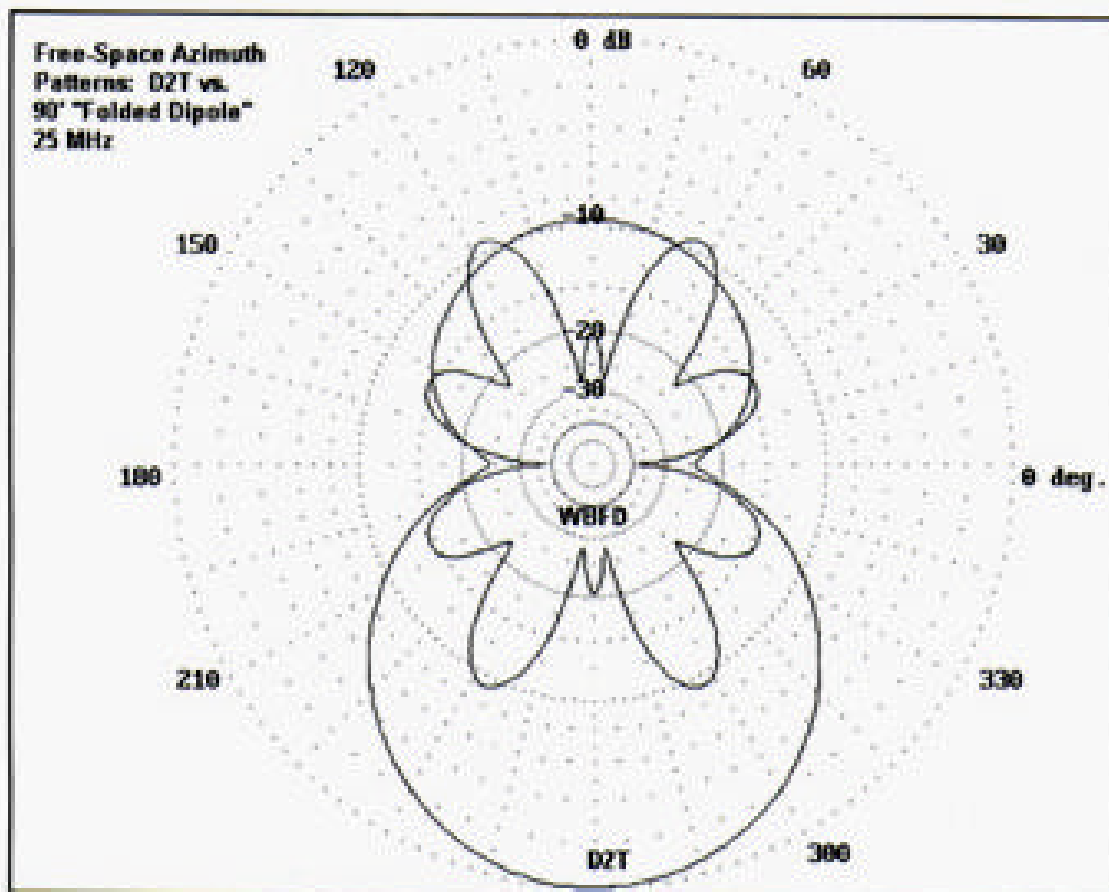
Fig. 6—Azimuth patterns at 25 MHz for the D2T and a standard 90 ft. "folded dipole" terminated horizontal antenna. Note the 9 dB gain differential at this frequency.
