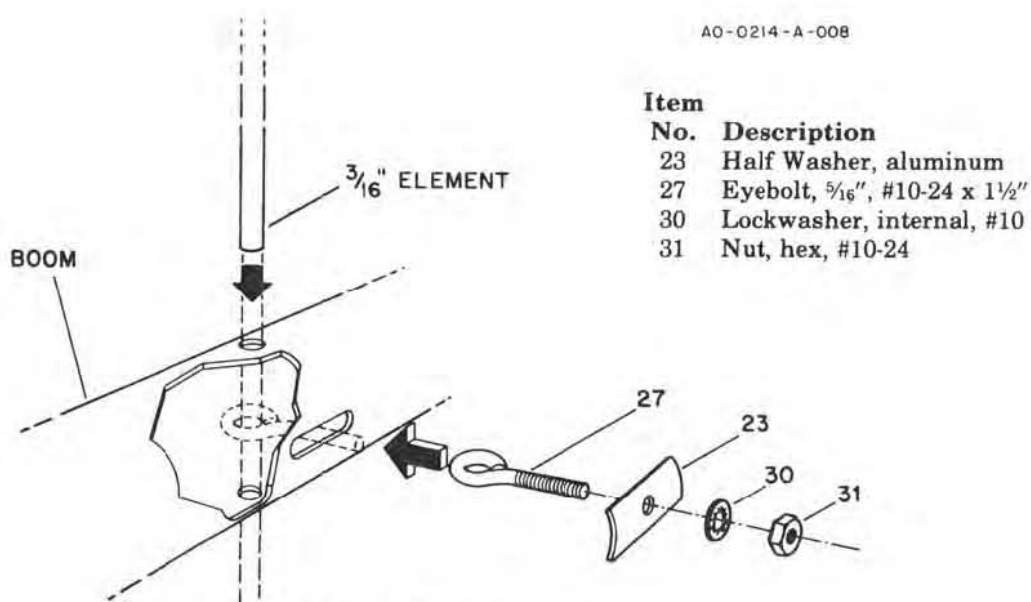
Figure 6 — Detail A Element Assembly
