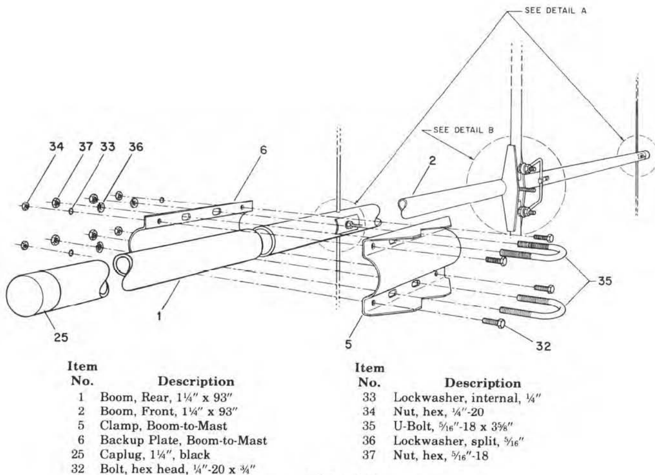
Figure 6 Boom-to-Mast Clamp Assembly
