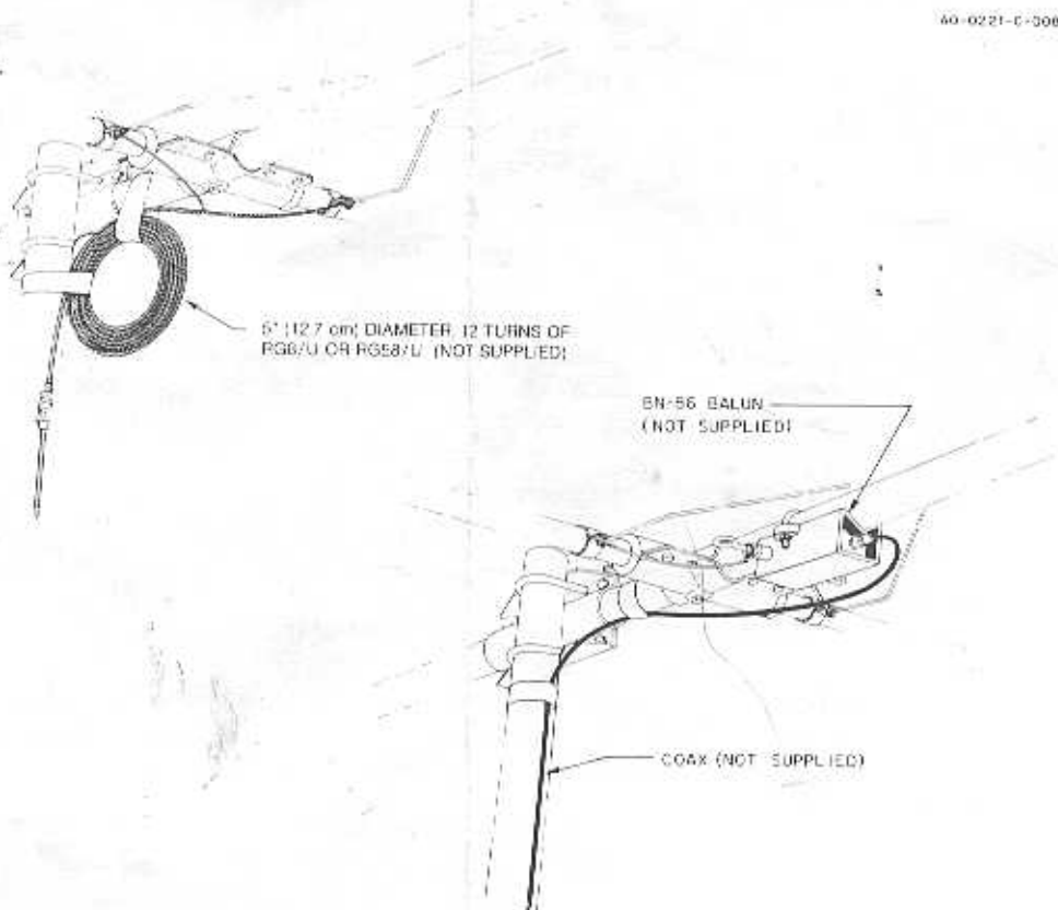
Figure 8. RF Choke
