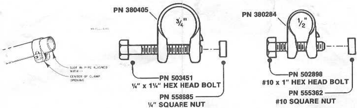
Figure 6 Compression Clamps
