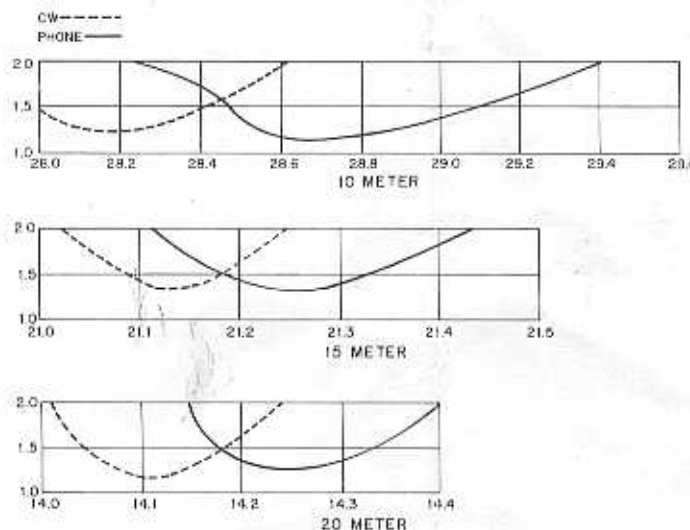
Figure 4. VSWR Chart
