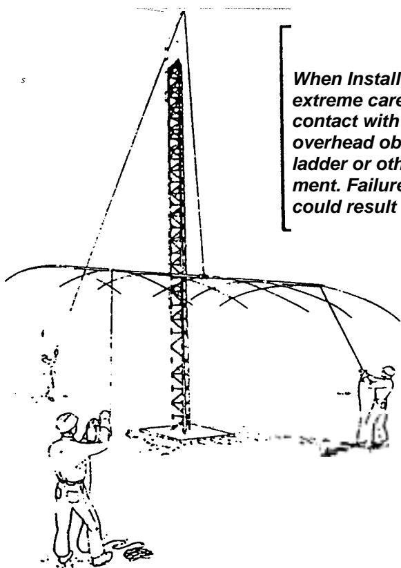
Complete Antenna Hoisted On Tower By Cable or Rope
