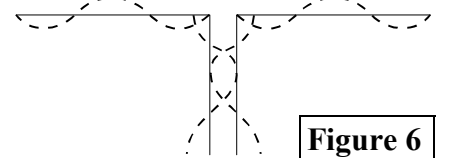
Current Distribution 21MHz
