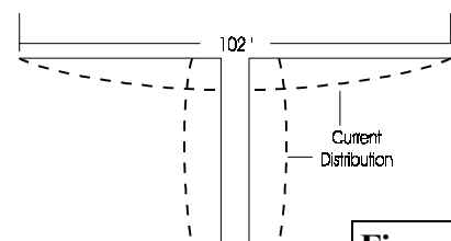
Current Distribution 3.5MHz
