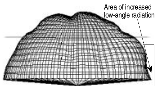
Figure 2 CAROLINA WINDOM 80
