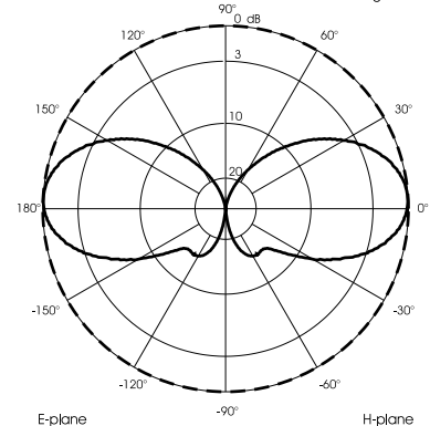
TYPICAL RADIATION PATTERN in E-plane at mid-band File: E-02-063 Scale: logarithmic
