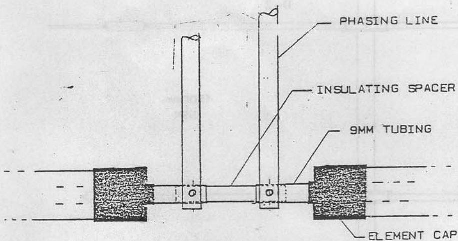
PHASING LINE ASSEMBLY ELEMENTS Ra AND Ref
