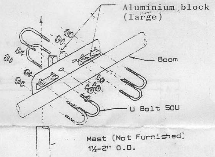
BOOM TO MAST BRACKET FIGURE 4
