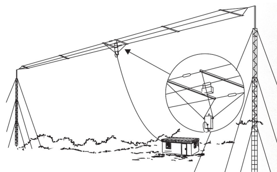
Horizontal configuration
