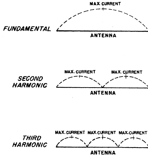
EXAMPLES OF RESONANT ANTENNA CURRENT DISTRIBUTIONS
