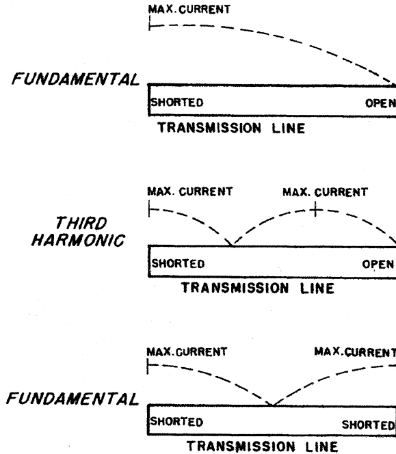
EXAMPLES OF RESONANT TRANSMISSION LINE CURRENT DISTRIBUTIONS
