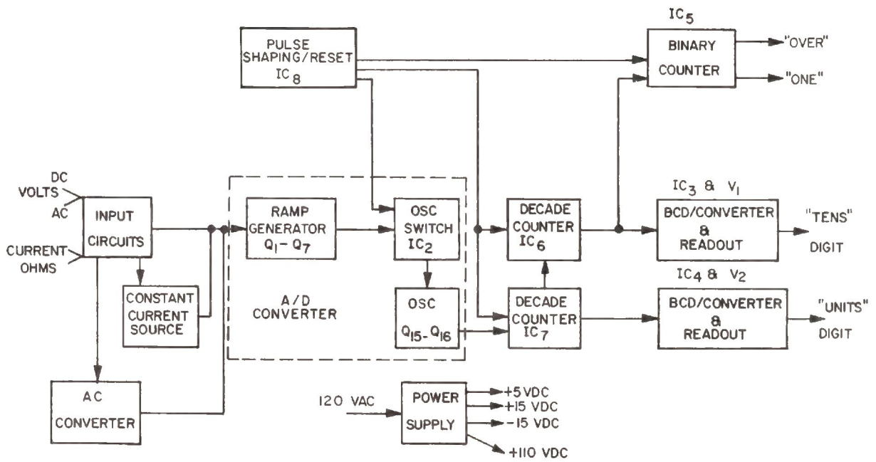
DMM BLOCK DIAGRAM FIGURE 1
