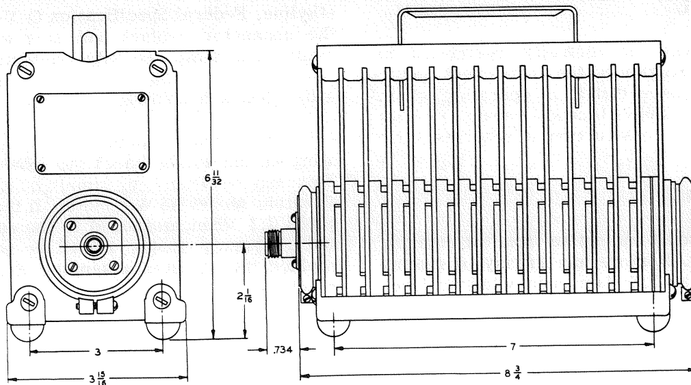
Figure 2-1. Mounting Dimensions
