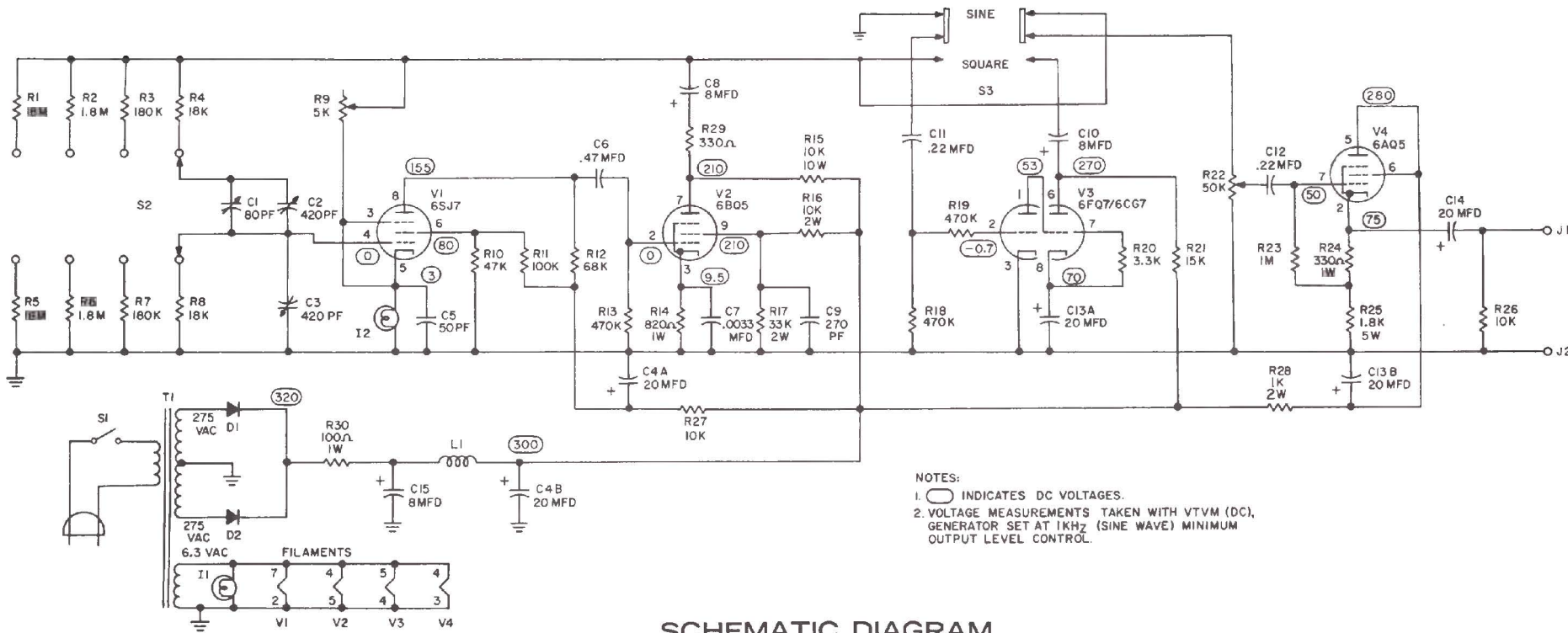
SCHMATIC DIAGRAM
