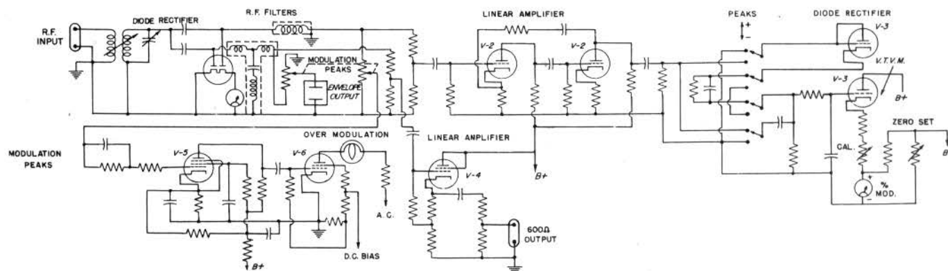
Figure 4. Elementary schematic circuit diagram.
