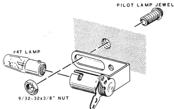
Detail 1H
