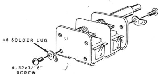
Detail 5A
