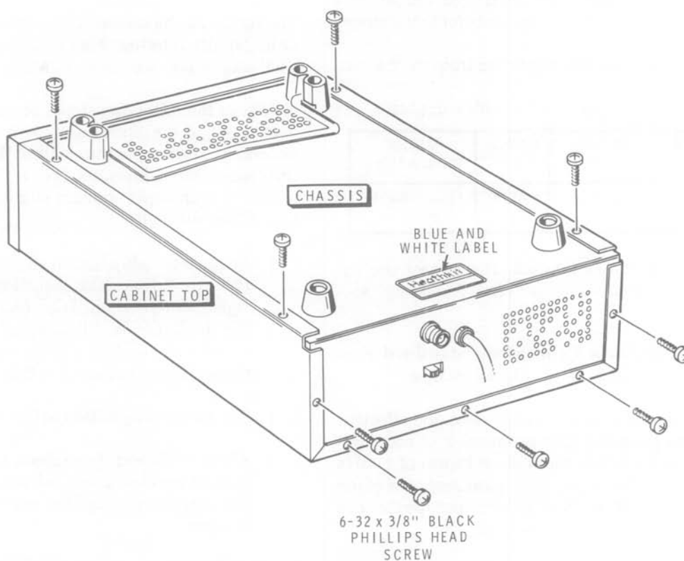
PICTORIAL 7-1
