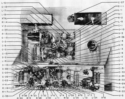
Figure 5.1 - Model 288X, Case Removed, Rear View
