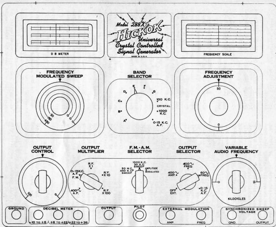
Figure 3.1 - Panel View, Model 288X
