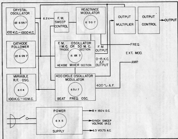
Figure 1.2 - Basic Circuit, Block Diagram, Model 288X
