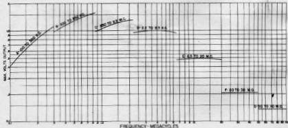
Figure 5.3 - Maximum Voltage Output
