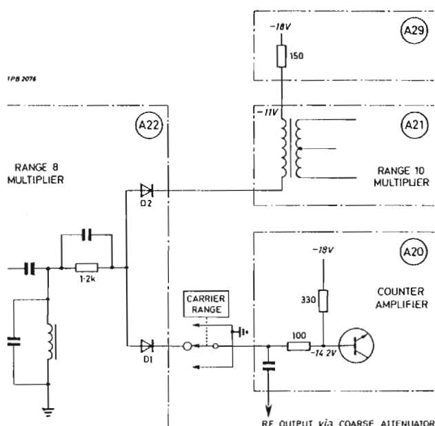
Fig. 3.2 Multiplier range switching
