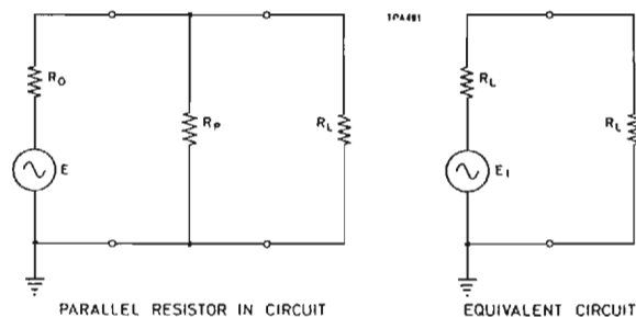
Fig. 2.10 Matching to low impedance loads
