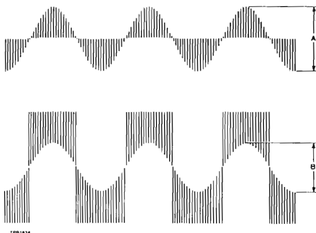
Fig. 4.16 Stereo waveforms
