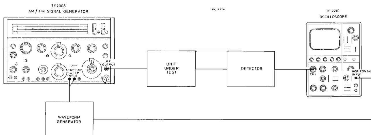
Fig. 2.7 Arrangement for narrow sweep
