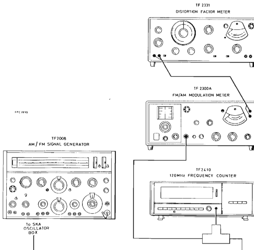
Fig. 5.1 Test gear arrangement to check FMO
