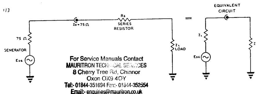
Fig. 2.11 Matching to High-Impedance Loads.
