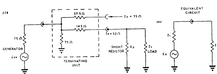
Fig. 2.10 Matching to Low-Impedance Loads.
