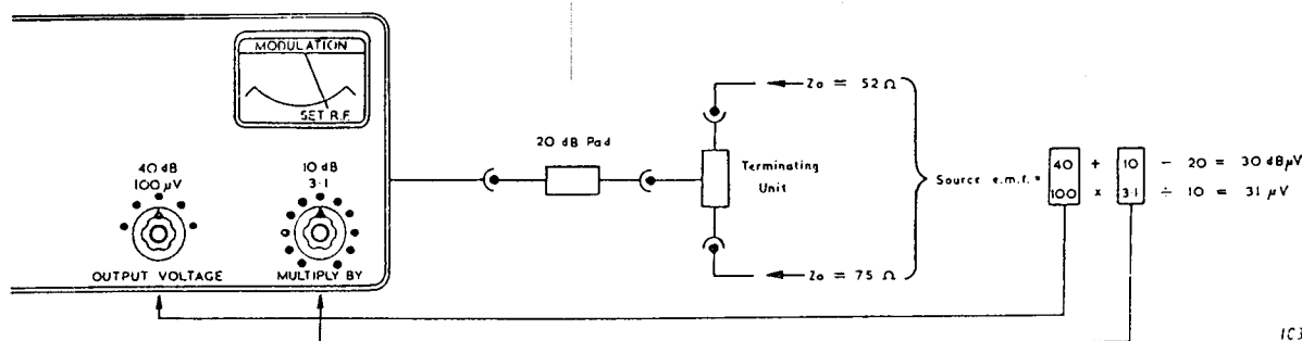
Fig. 2.9 Outputs via 20-dB Pad and Terminating Unit.
