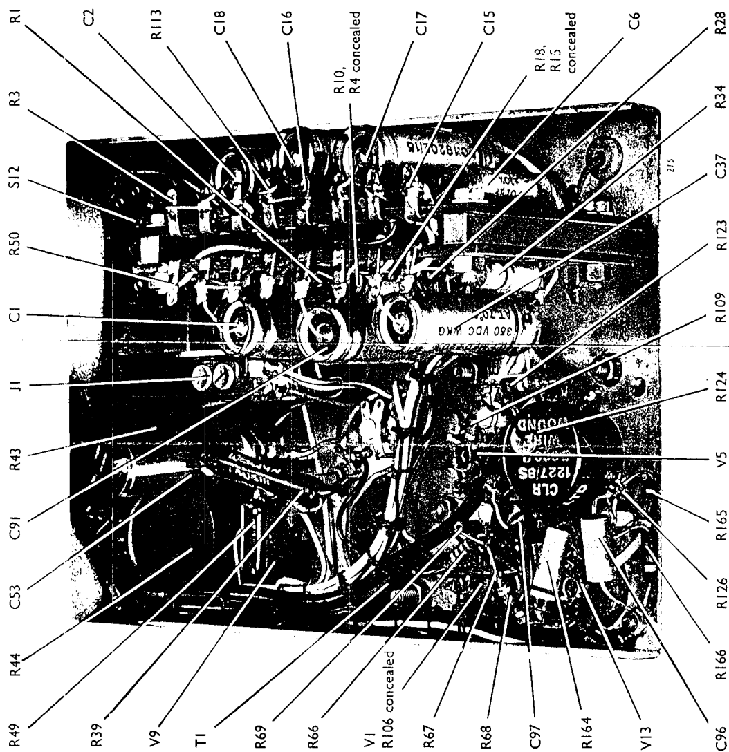
L.F. UNIT UNDERSIDE VIEW
