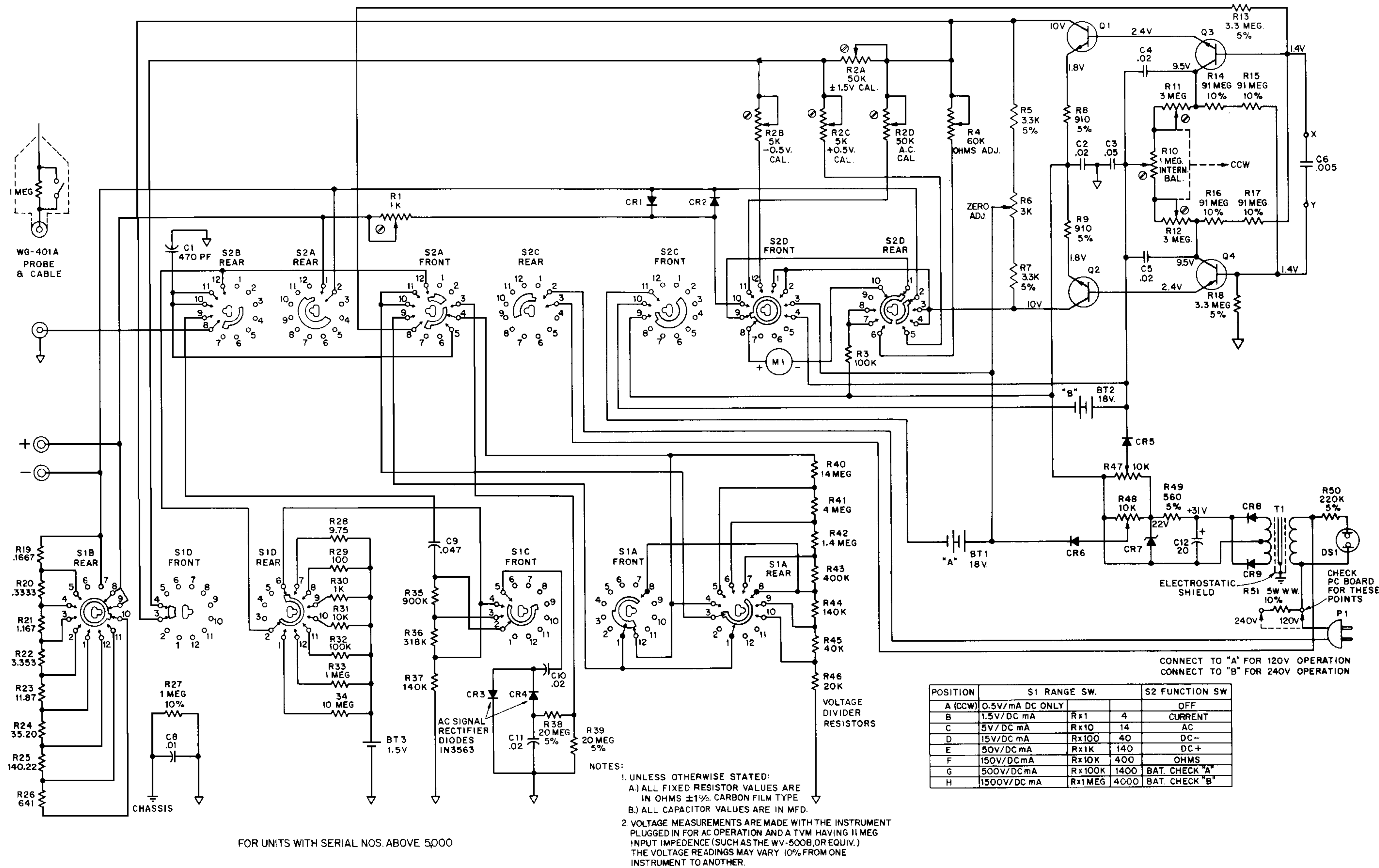
WV-510A Schematic Diagram
