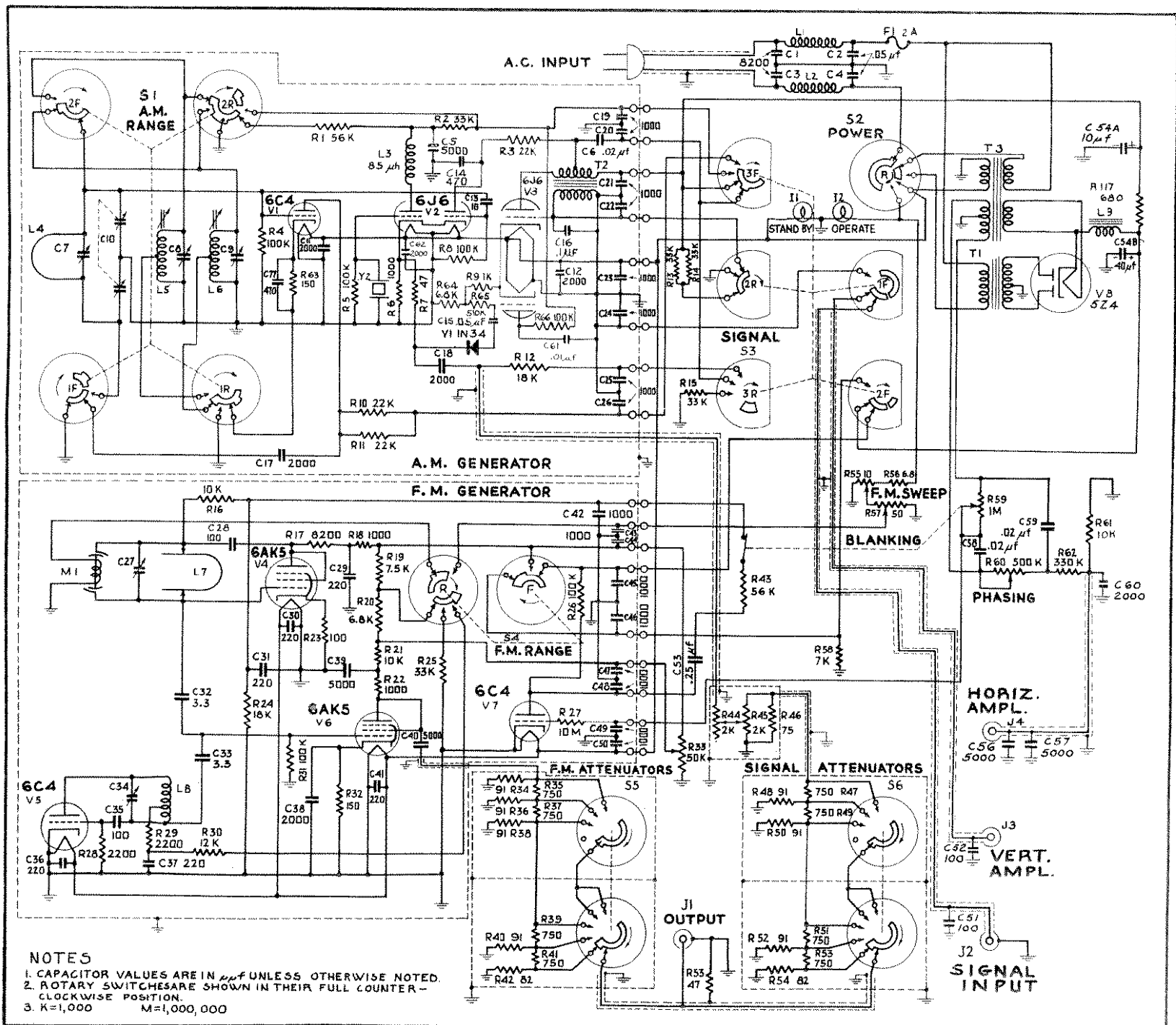
FIG. 19. MODEL 479 SCHEMATIC DIAGRAM
