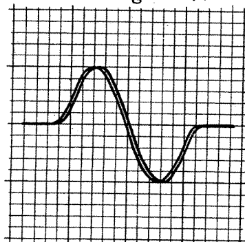
FIG. 9. DISCRIMINATOR RESPONSE - IN PHASE - BLANKING OFF
