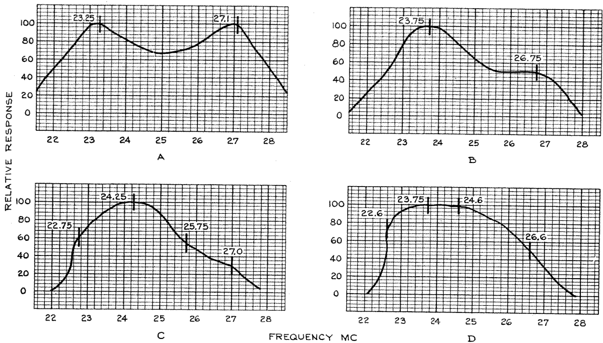
FIG. 6 VIDEO ALIGNMENT CURVES - BAND PASS TYPE
