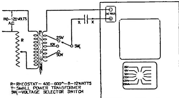
MODEL 772 ANALYZER
