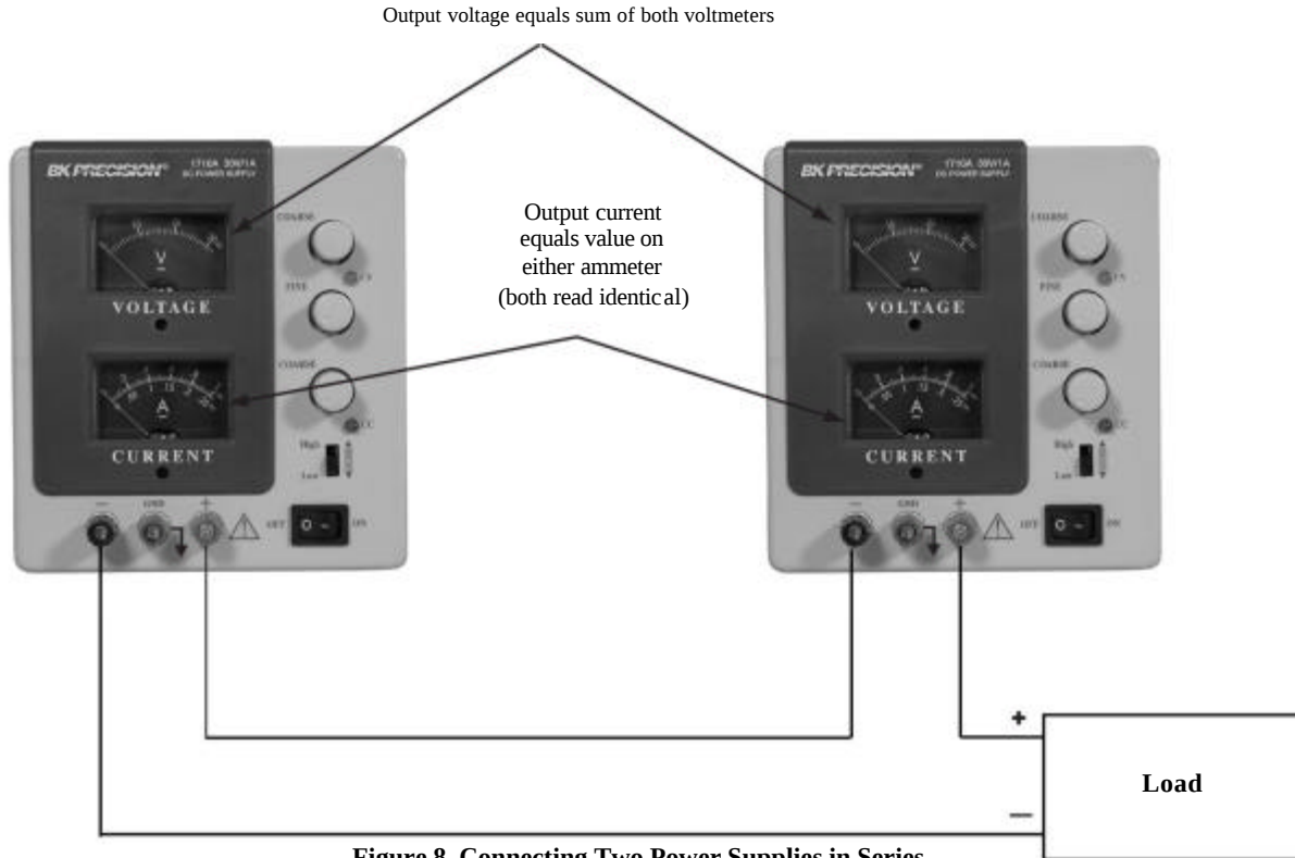
Figure 8. Connecting Two Power Supplies in Series.
