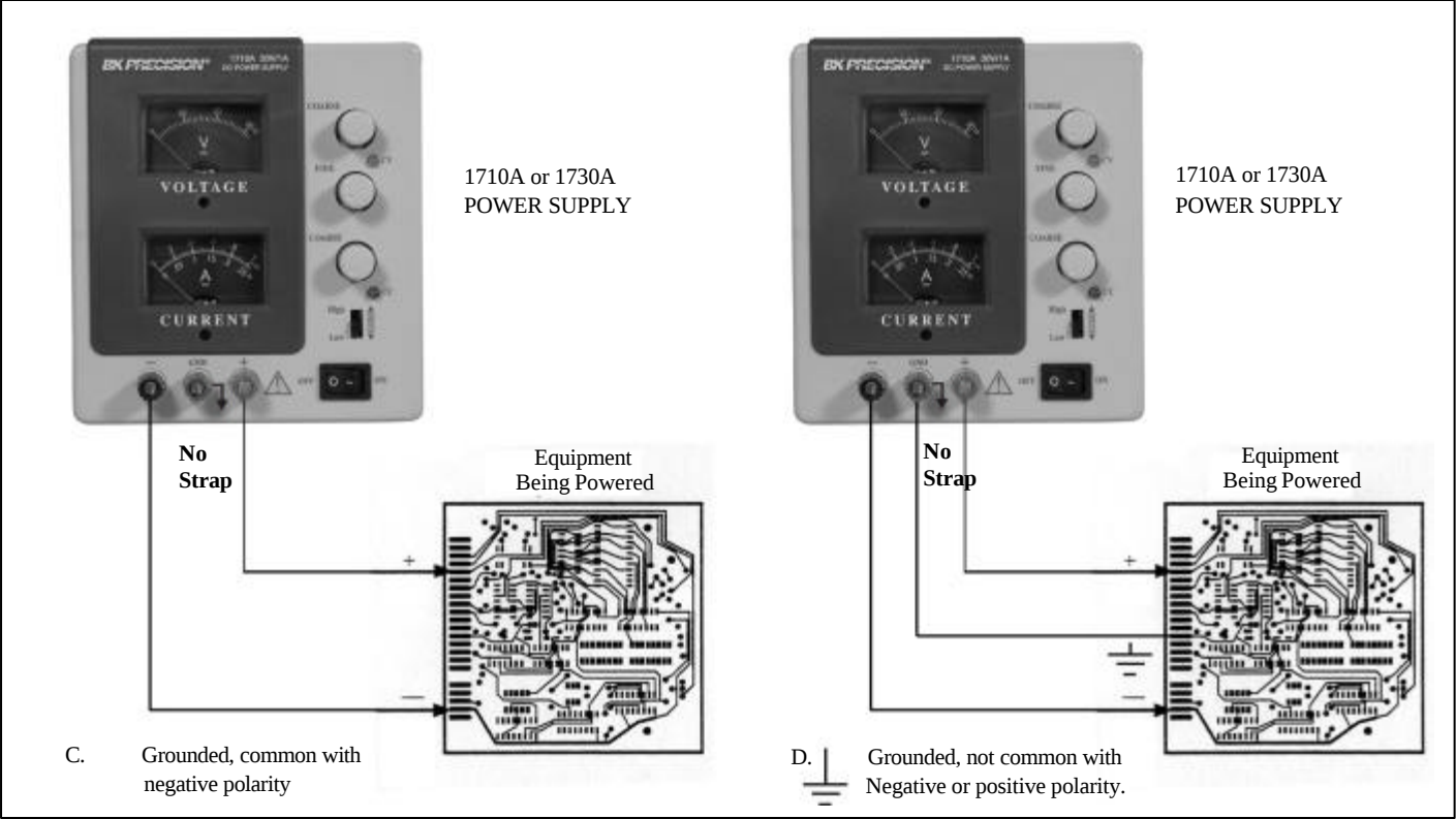
Figure 3 (C and D). Grounding Possibilities.
