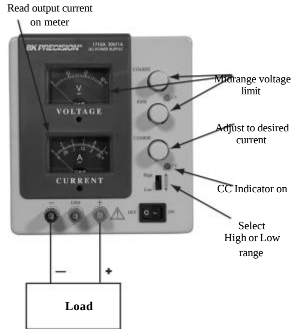
Figure 6. Typical Constant Current Operation.
