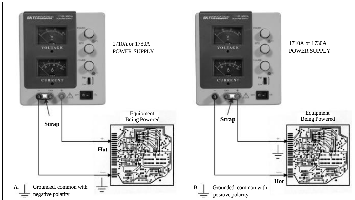
Figure 3 (A and B). Grounding Possibilities.
