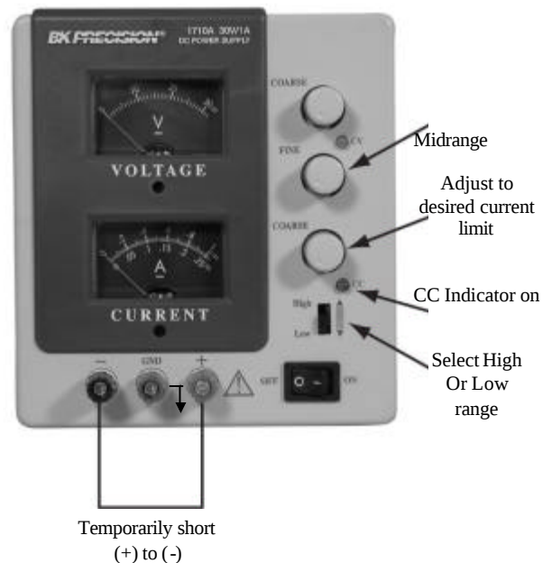
Figure 5. Setting Current Limit.
