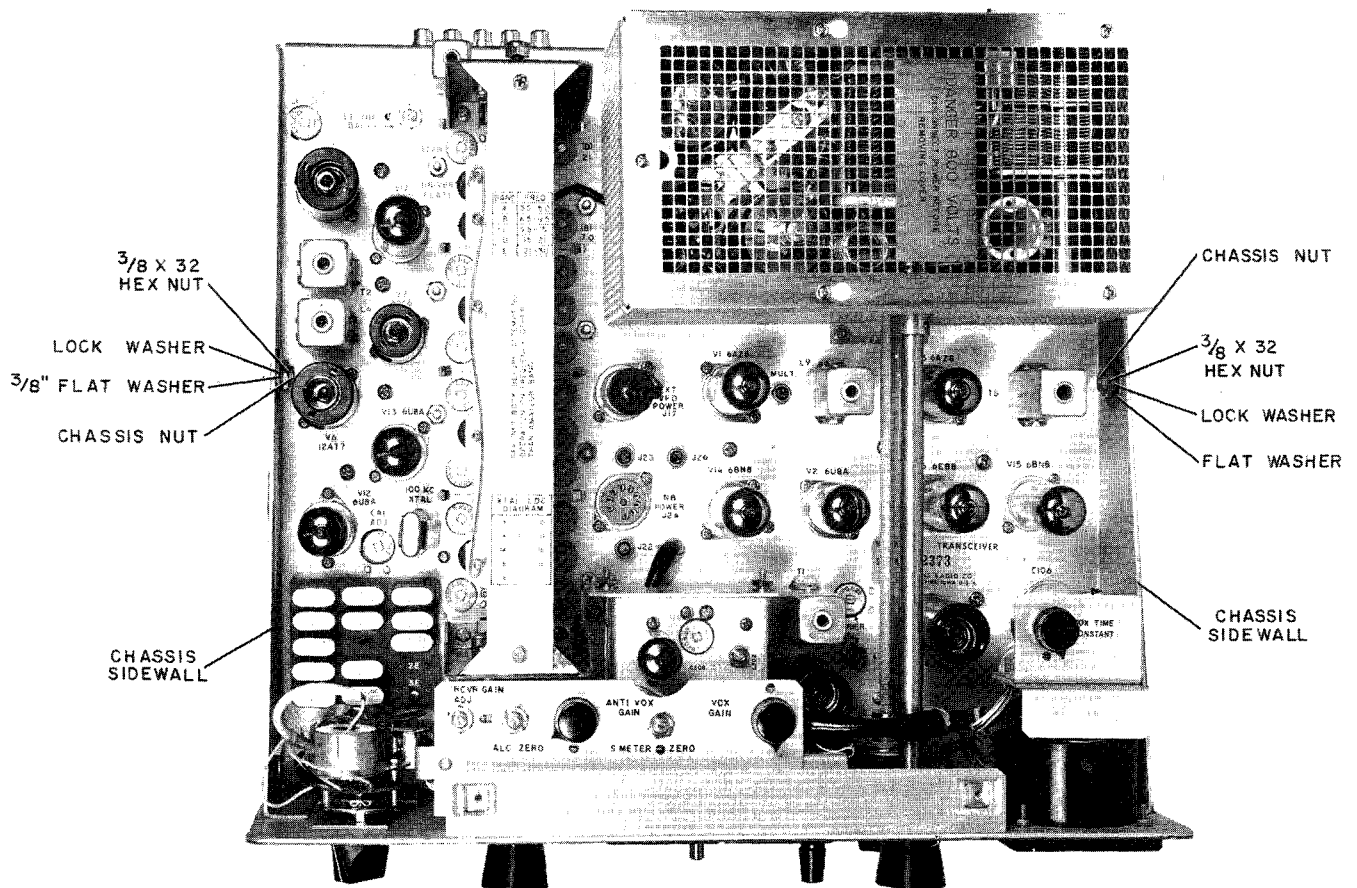
Figure 2. Installation of Chassis Nuts
