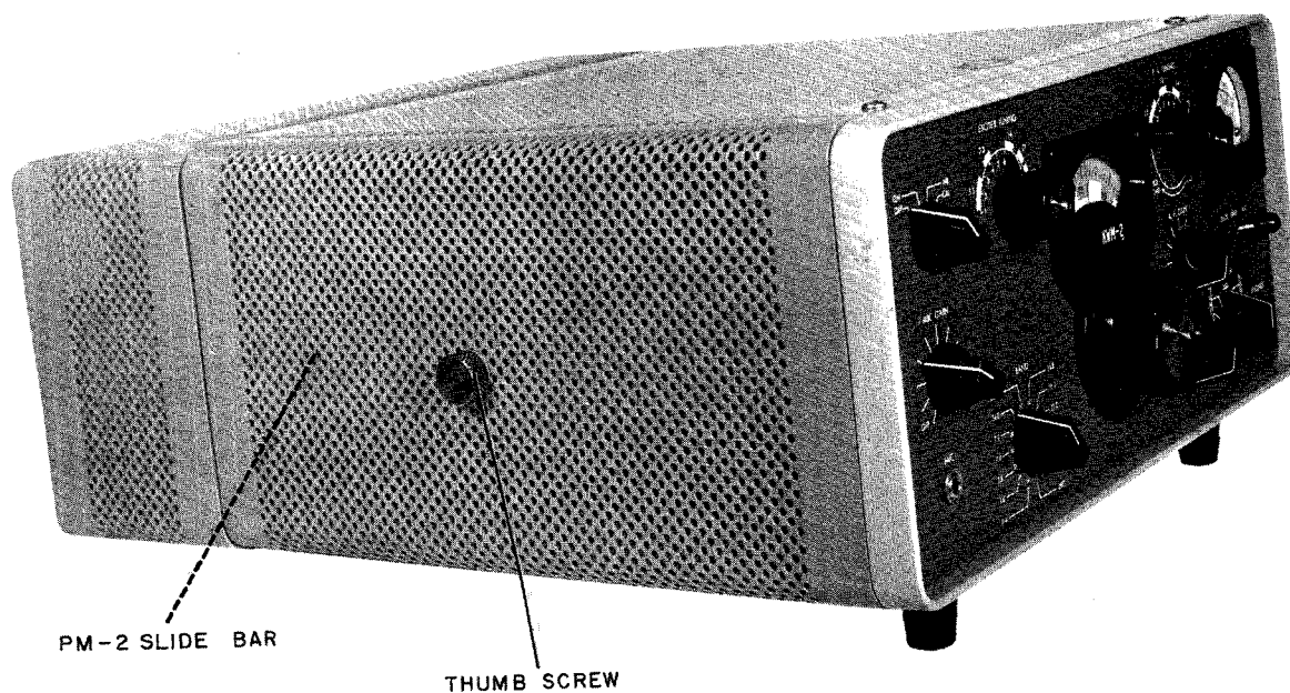
Figure 4. PM-2 Assembled to KWM-2
