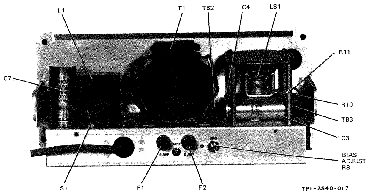
Figure 6. Top Chassis Parts Location
