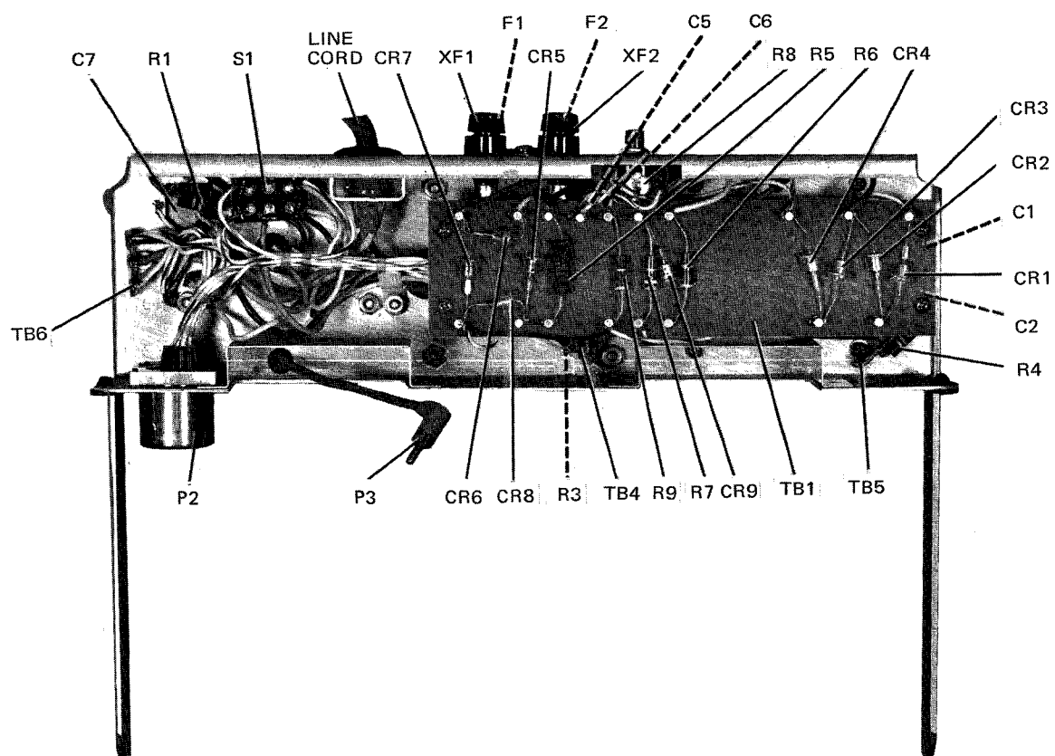
Figure 7. Bottom Chassis Parts Location
