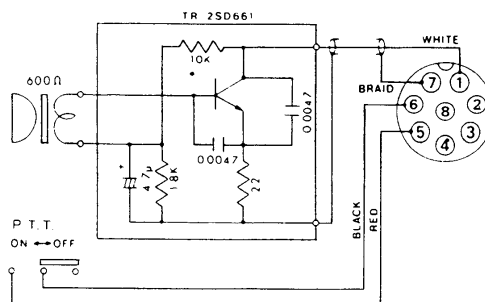
Schematic diagram of IC-SM5
