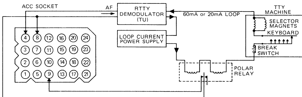
When a high speed relay is used
