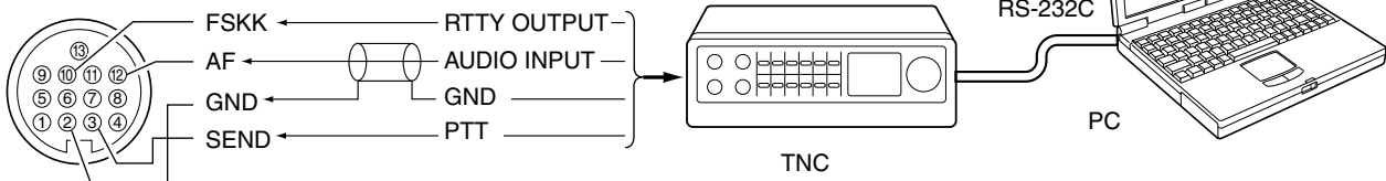
Rear panel view
