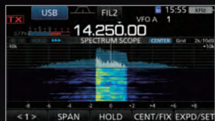
DPD OFF (Signal Received on the IC-7300)
