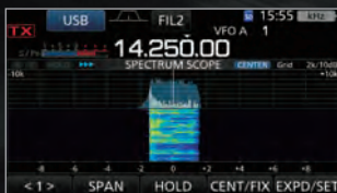
DPD ON (Signal Received on the IC-7300) No spurious emission observed
