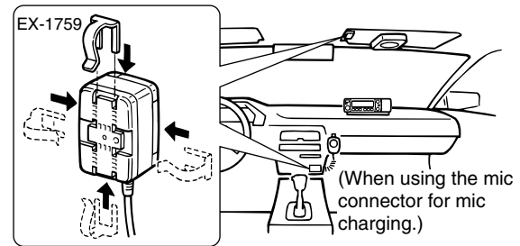
The installation clip can be oriented in 1 of 4 ways.
