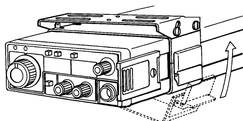
Transceiver installation
