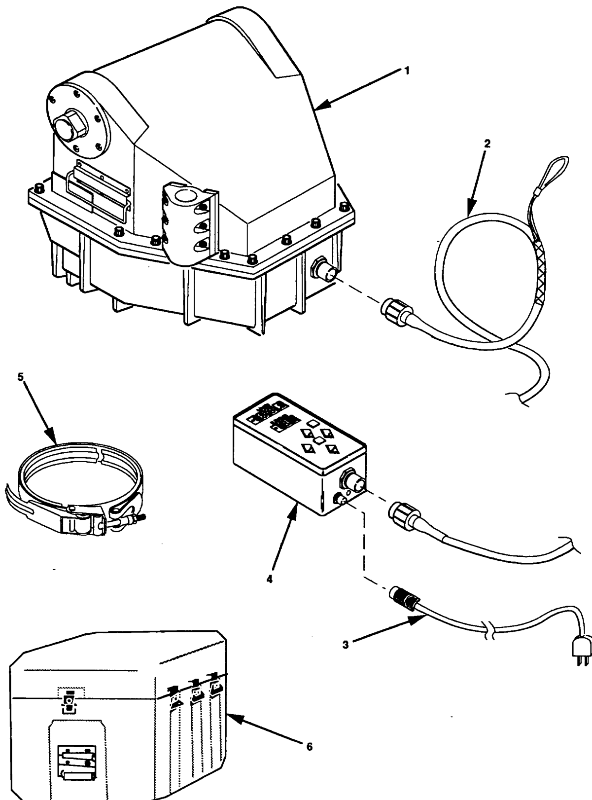
Figure 10. Positioner System
