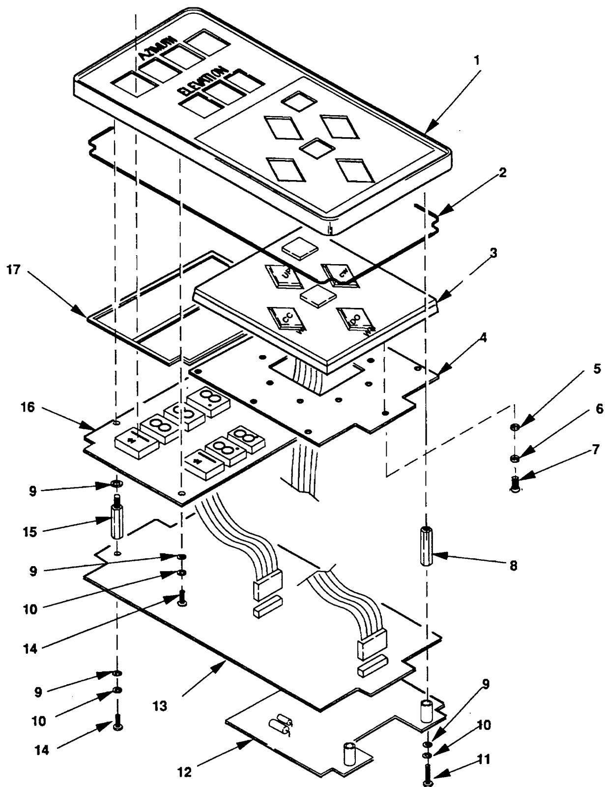
Figure 12. Front Panel
