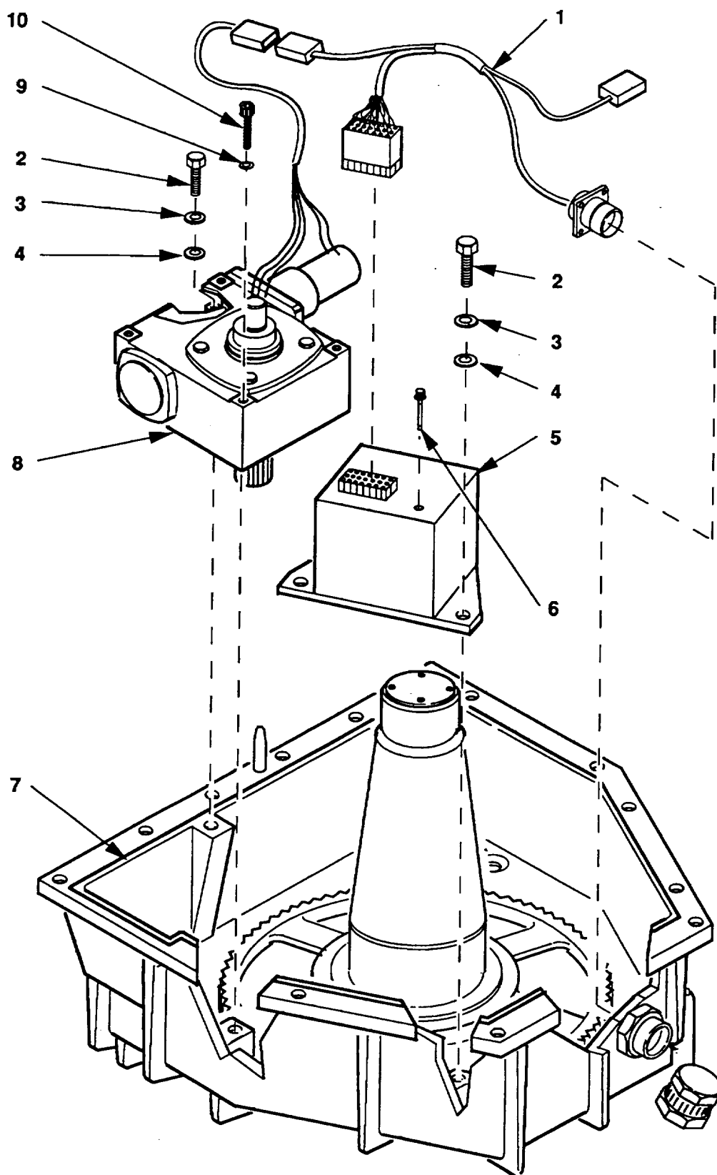
Figure 14. Azimuth Assembly (Sheet 1 of 2)
