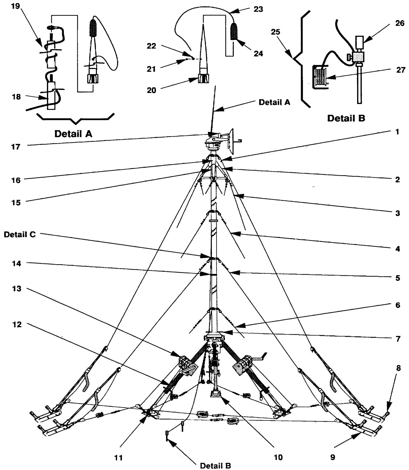
Figure 2. Mast Assembly (Sheet 1 of 3)
