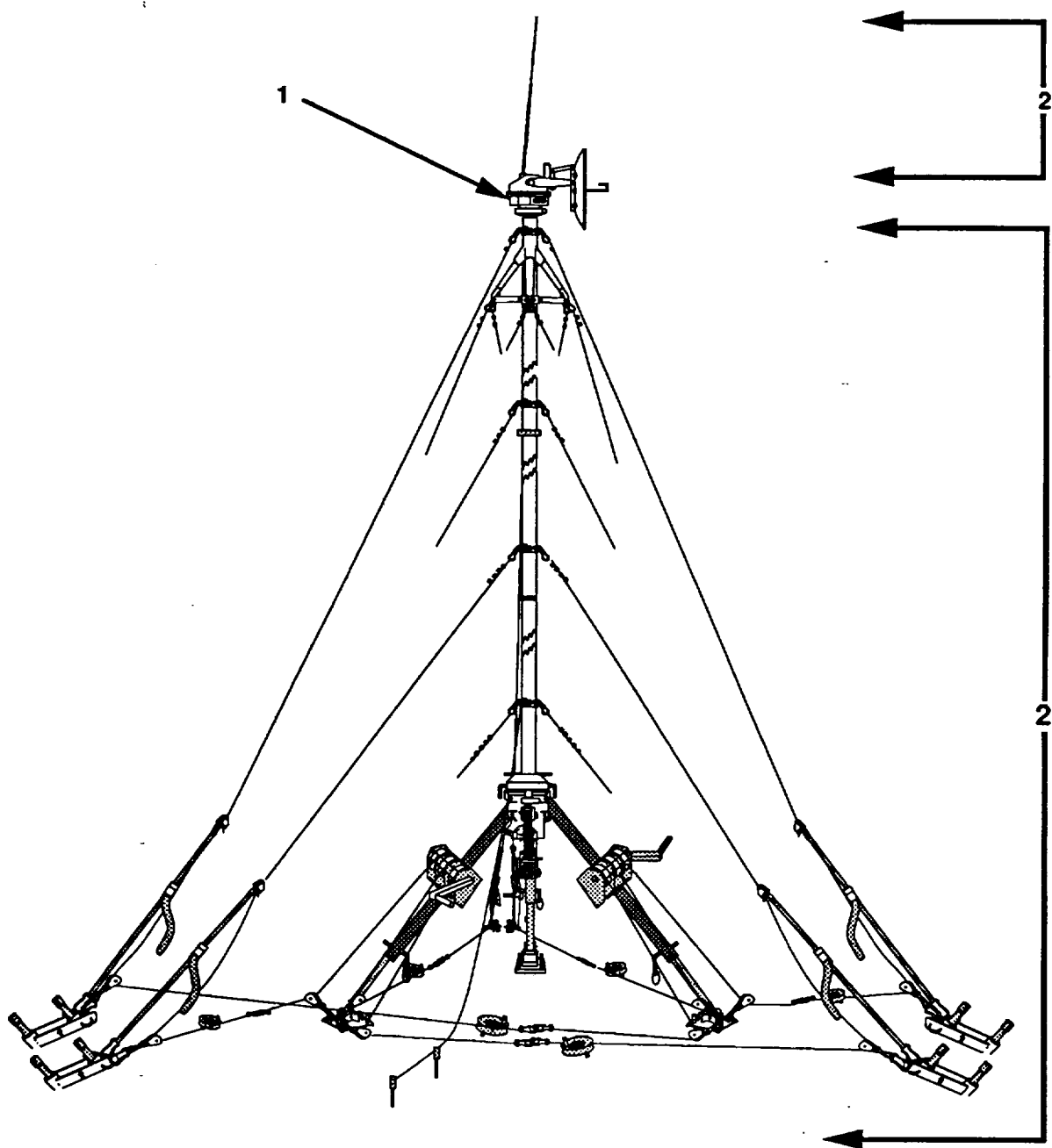
Figure 1. Mast AB-1373/TRC
