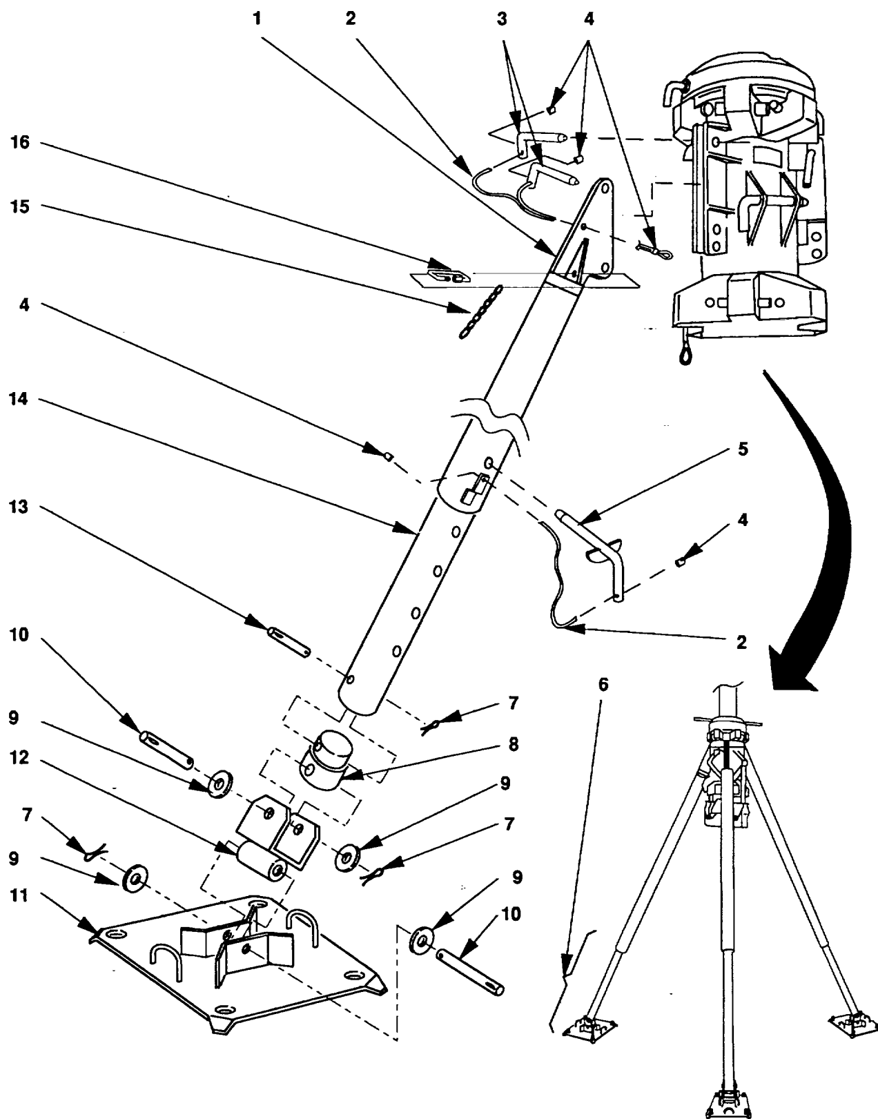
Figure 5. Support, Antenna
