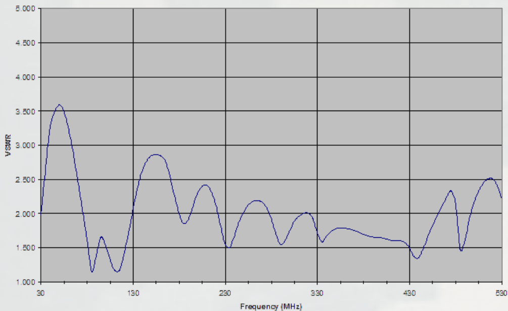
SF3512 VSWR
