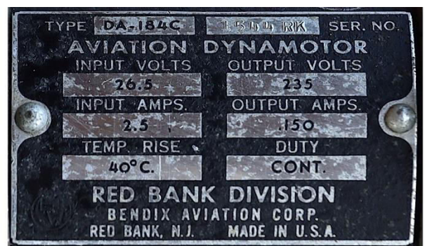
Figure 7. Dynamotor nameplate
