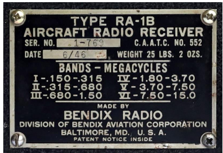
Figure 1. RA-1B nameplate
