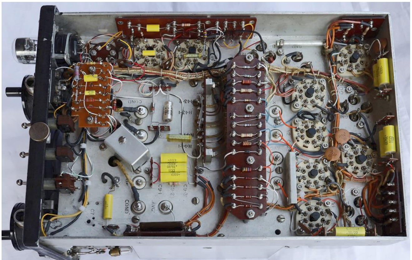
Figure 4. RA-1B: Under-chassis view of the refurbished radio
