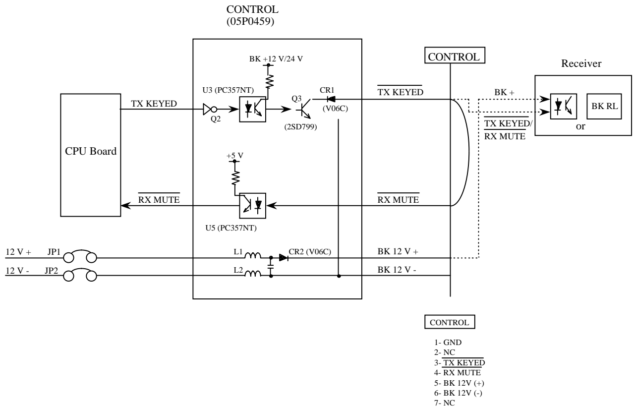
Figure 2-29 CONTROL Board
