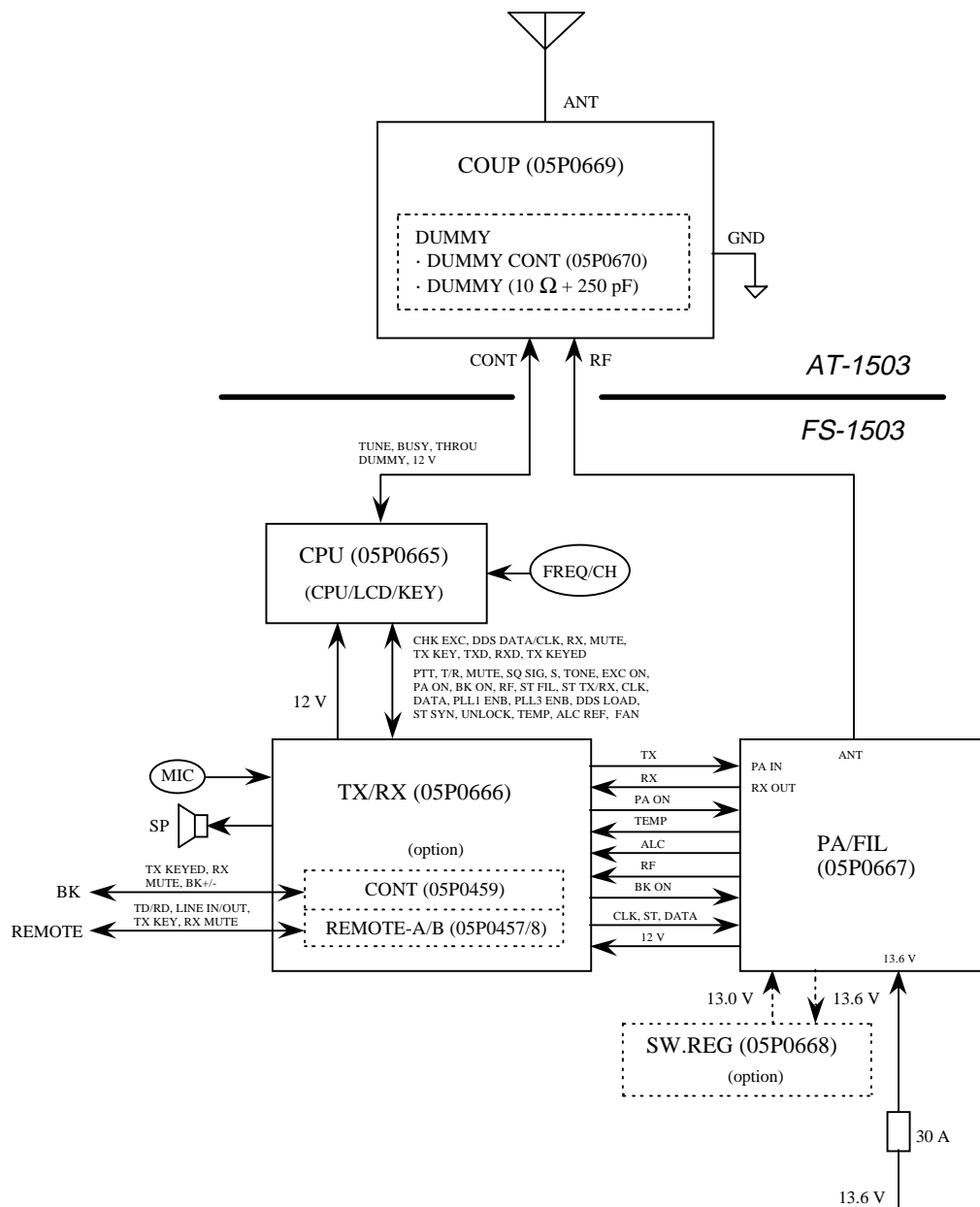
Figure 2-1 Interconnection Diagram
