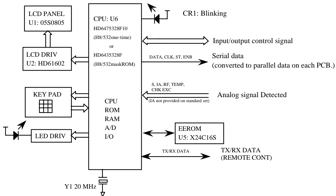
Figure 2-2 Block Diagram of CPU
