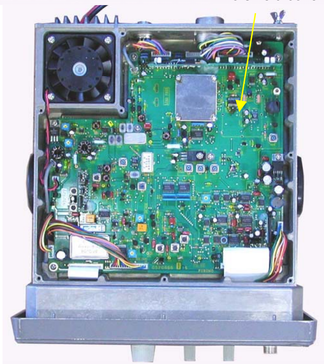
Fig.5 TX/RX board, 05P0666B/C
