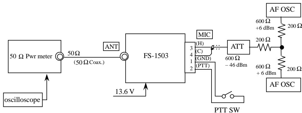
Figure 5-4 Measurement of TX output power
