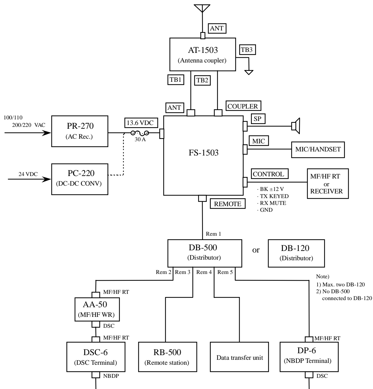
Figure 1-1 System Diagram
