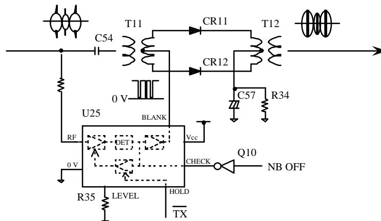
Figure 2-16 NB Circuit
