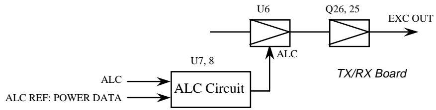
Figure 2-13 ALC Signal
