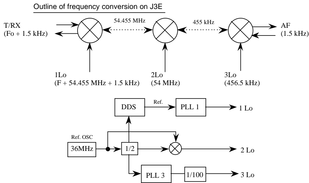
Figure 2-6 Frequency Conversion
