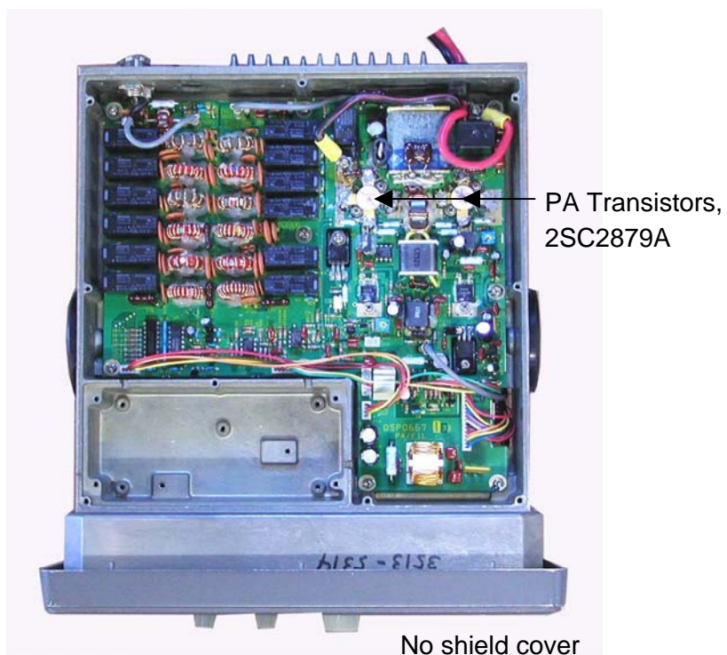
Fig.4 PA/FIL board, 05P0667A
