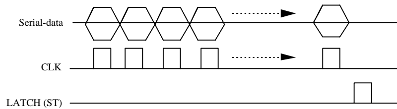
Figure 2-4 Transmission Timing
