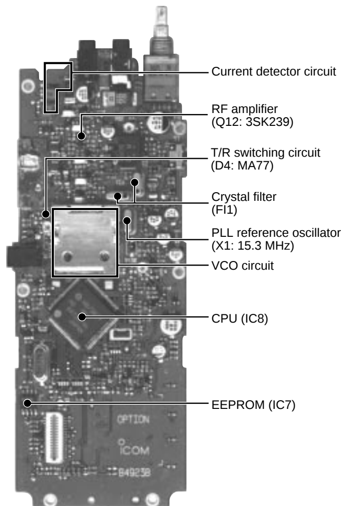
BOTTOM VIEW
