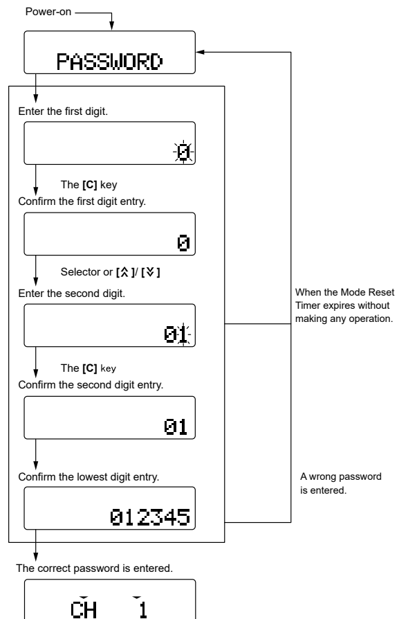
Figure 5-1 Transceiver Password Operation
