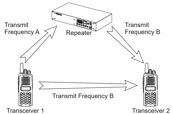
Figure 13-1 Talk Around
