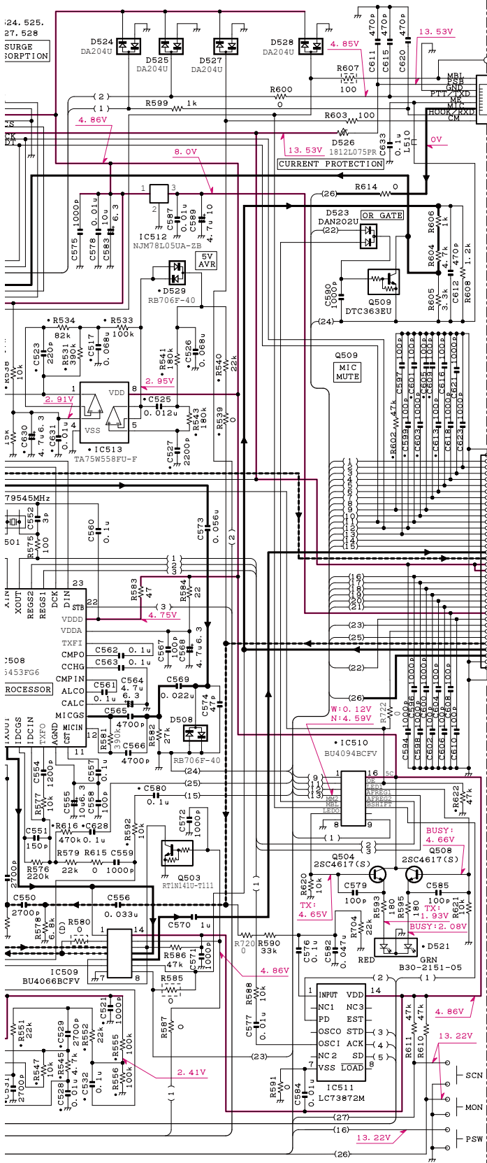
-RX UNIT(X57-5950-XX) (B/2):CONTROL SECTION
