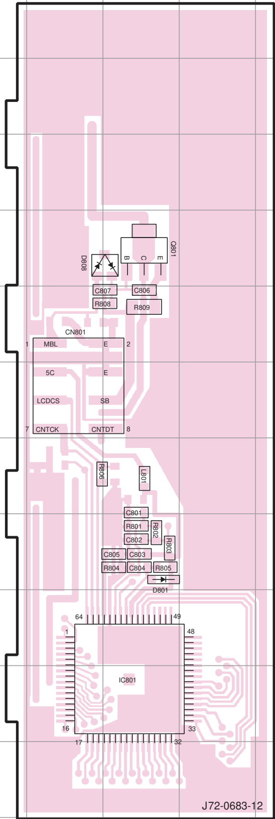
DISPLAY UNIT (X54-3270-10) Foil side view (J72-0683-12)
