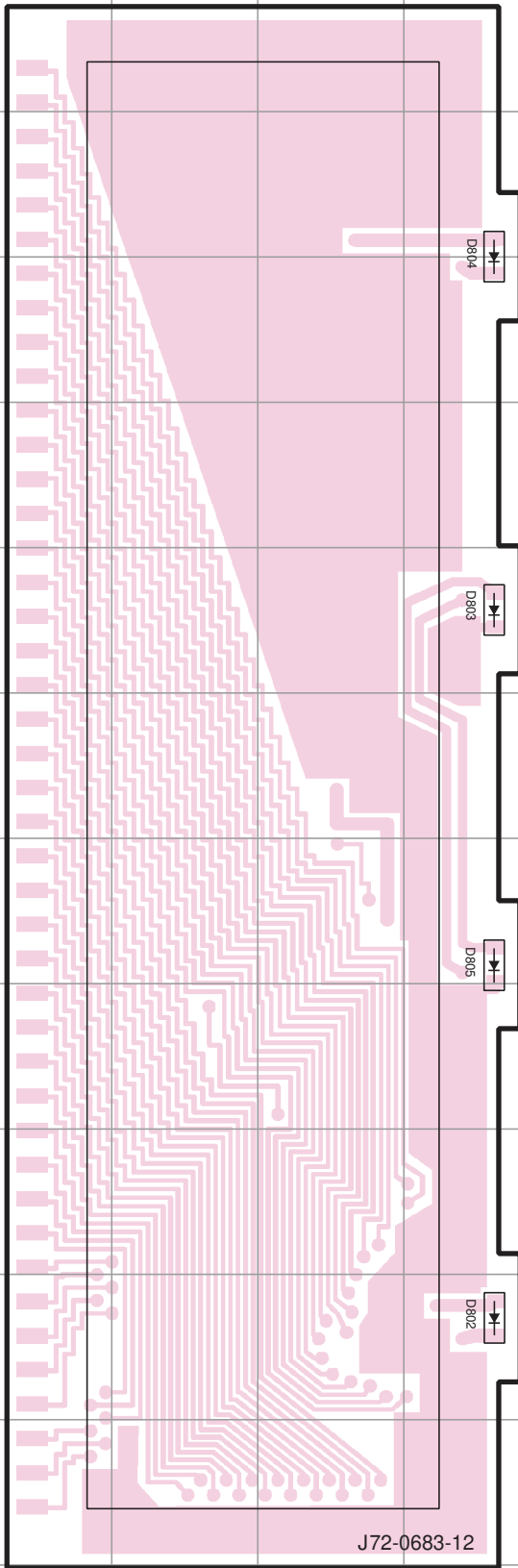
DISPLAY UNIT (X54-3270-10) Component side view (J72-0683-12)
