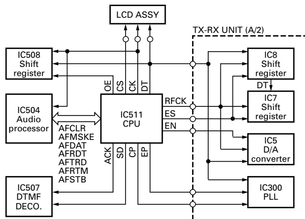
Fig. 8 Control circuit
