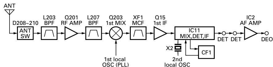
Fig. 2 Receiver system
