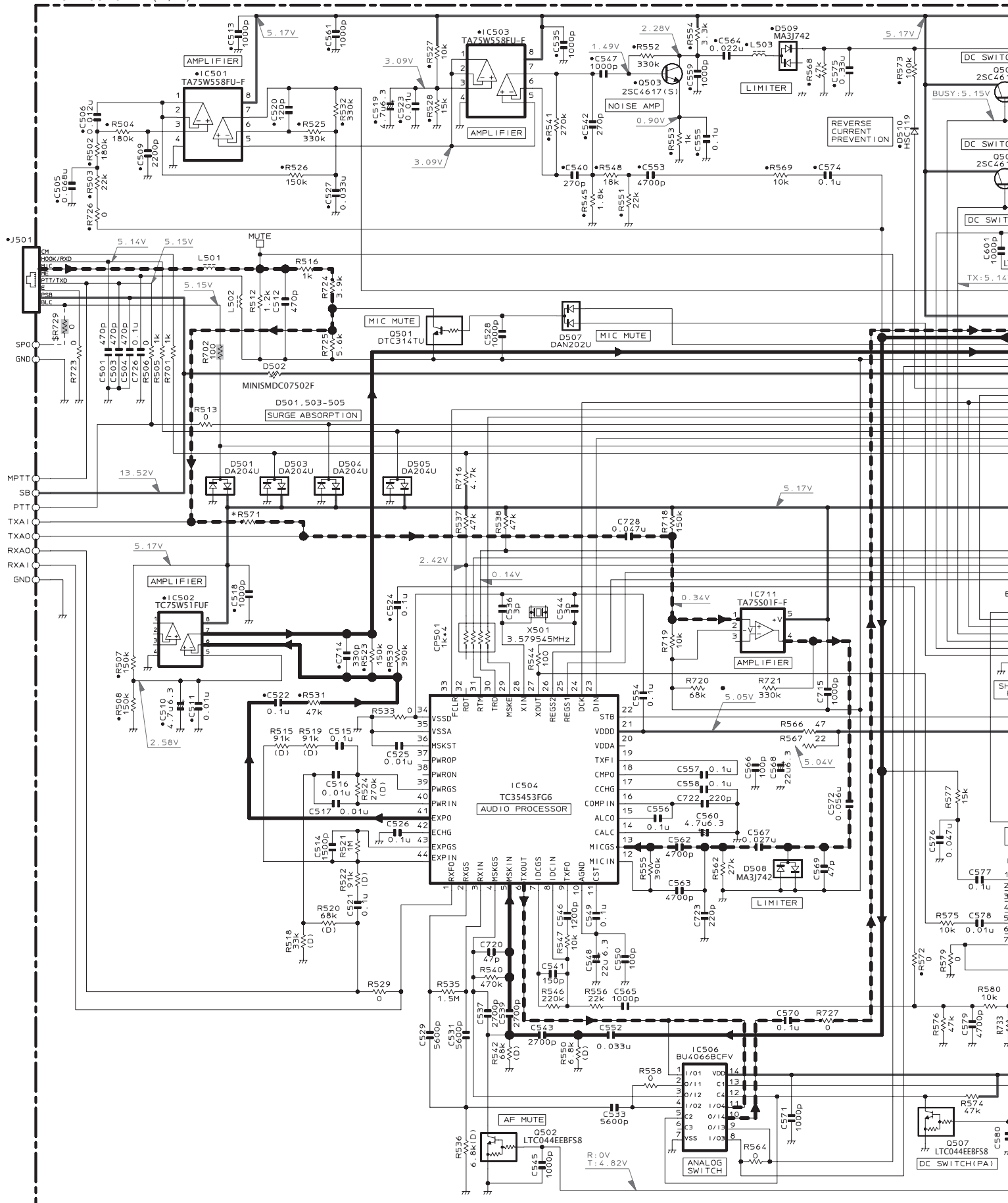
X57-6520-XX (B/2) TX-RX UNIT CONTROL SECTION
