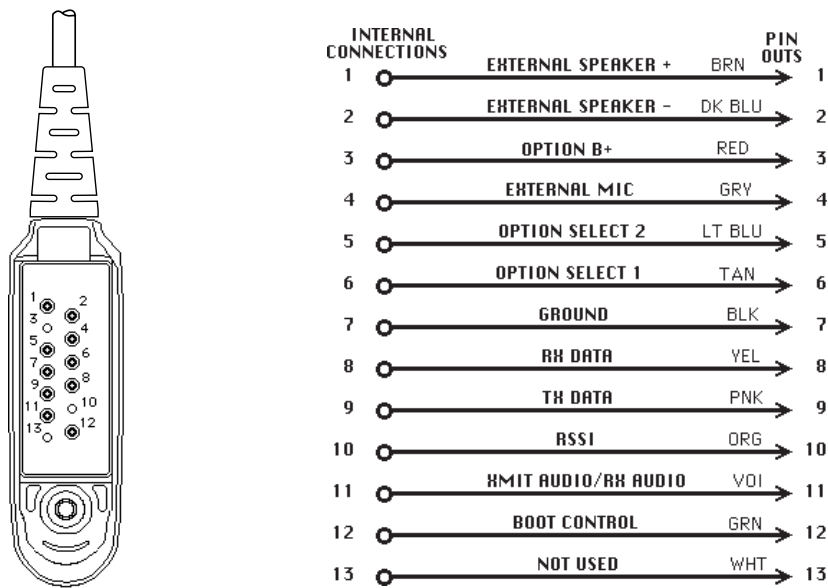
Figure 3-23: Pin Configuration of the Cable Side Connector
