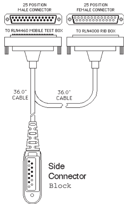
Figure 3-22: Programming/Test Cable AARKN4074
