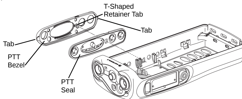
Figure 3-7: PTT Removal
