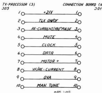
CABLE 3 : TX-PROCESSOR TO CONNECTION BOARD
