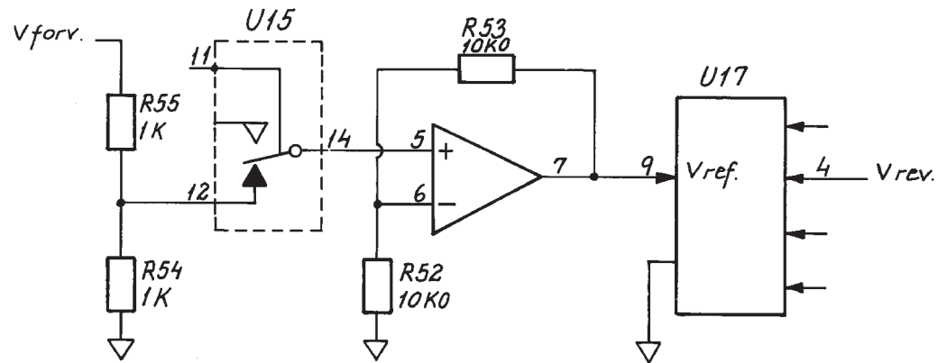
Figure 6: Measuring RHO
