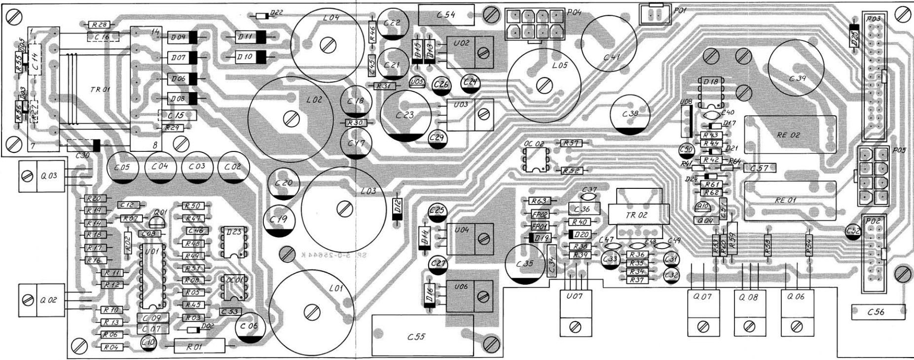
Seen from component side with lower side tracks. PCB rev. 25644K
