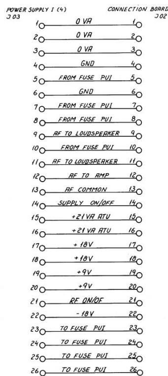
CABLE 5 : POWER SUPPLY I TO CONNECTION BOARD
