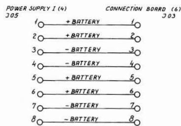
CABLE 4 : POWER SUPPLY I TO CONNECTION BOARD
