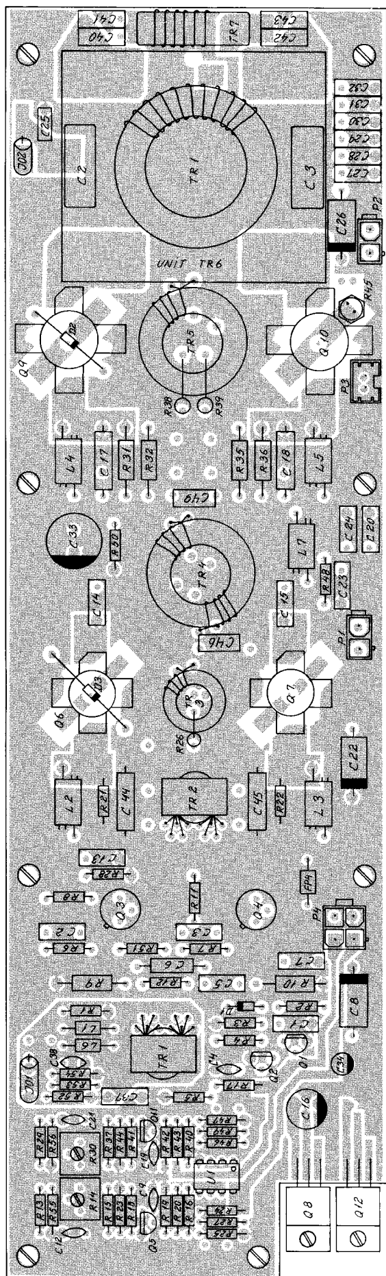
Seen from component side with upper side tracks PCB rev. 256411
