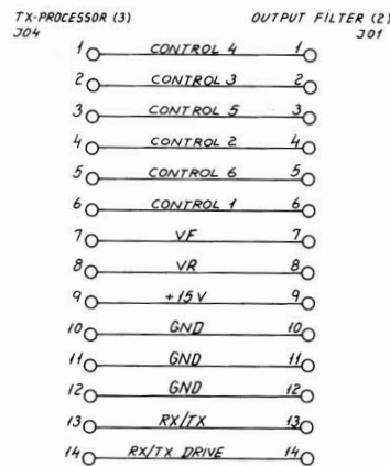
CABLE 2 : TX-PROCESSOR TO OUTPUT FILTER
