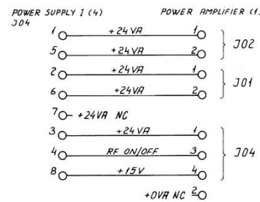
CABLE 7 : POWER SUPPLY I TO POWER AMPLIFIER
