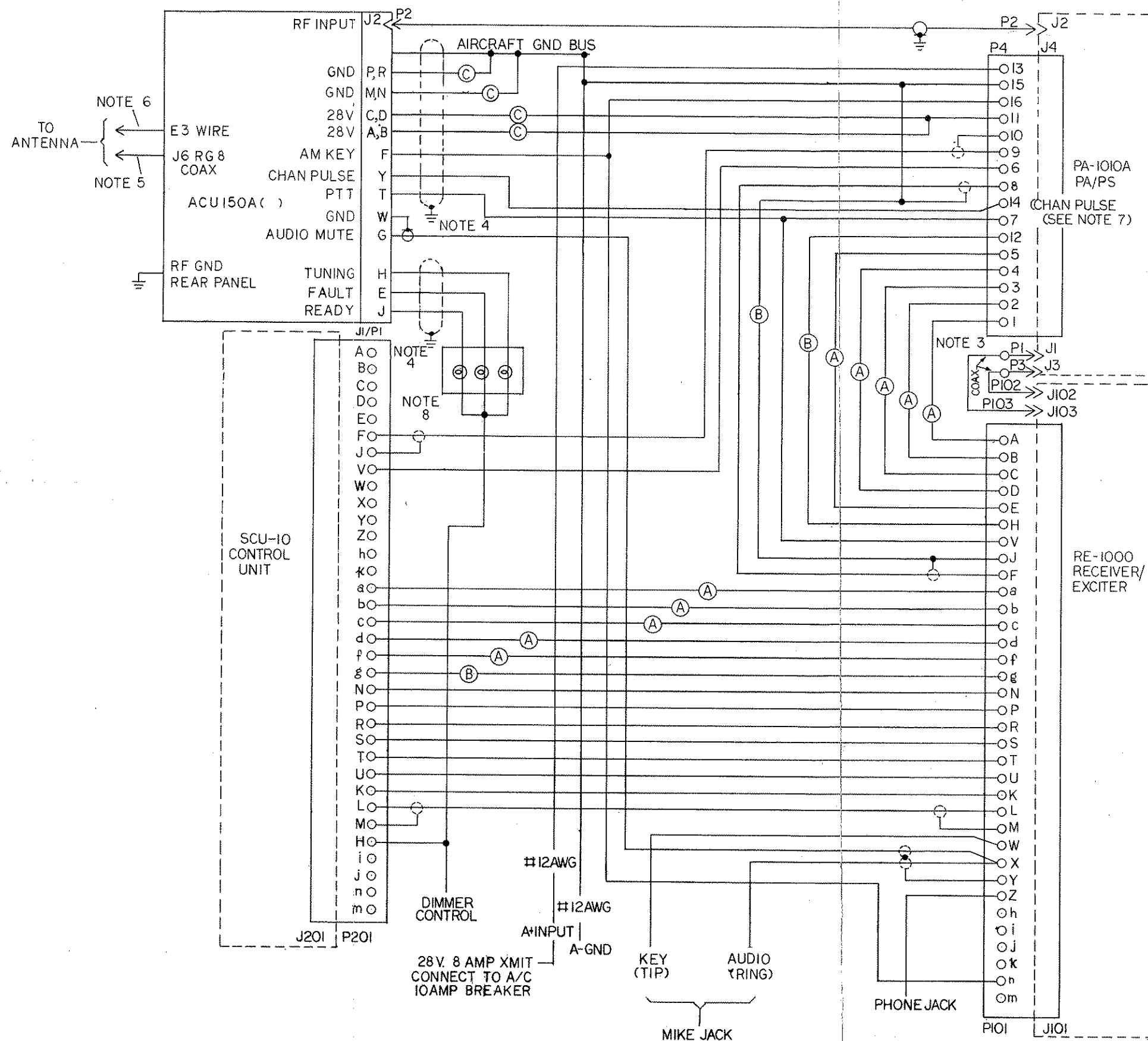
Figure 2.6. Interconnect Diagram, ASB-100A/ACU-150A ( ) System
