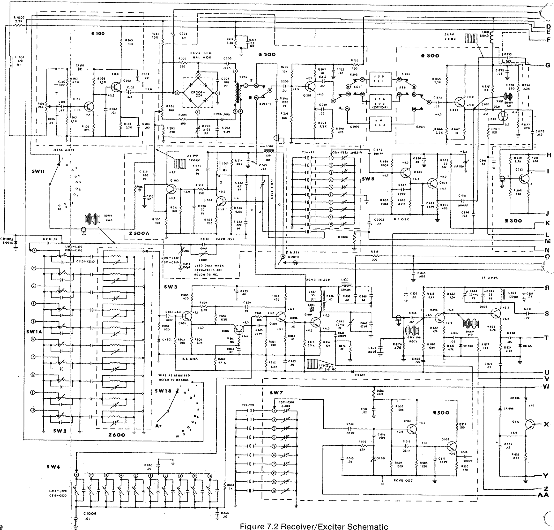
Figure 7.2 Receiver/Exciter Schematic
