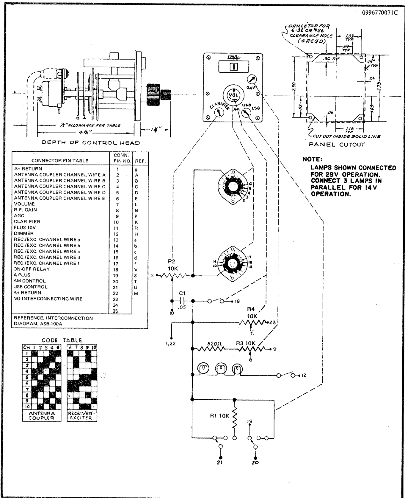
Figure 2.5. MCU-30, ASB-100A, Control Head Schematic and Mounting Diagram
