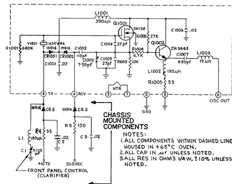
Figure X-20 - P.C. #10, 1650 OSCILLATOR
