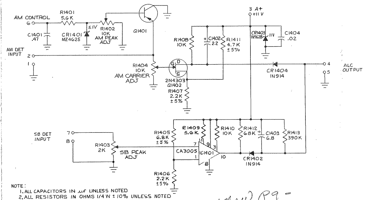
Figure X-17 - ALC DETECTOR AND AMPLIFIER
