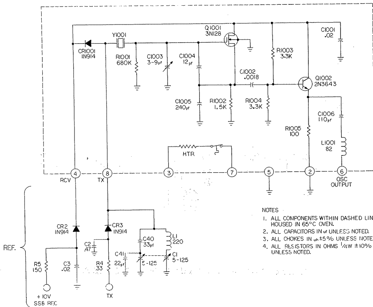
Figure X-20 1- P.C. #10, 1650 OSCILLATOR
