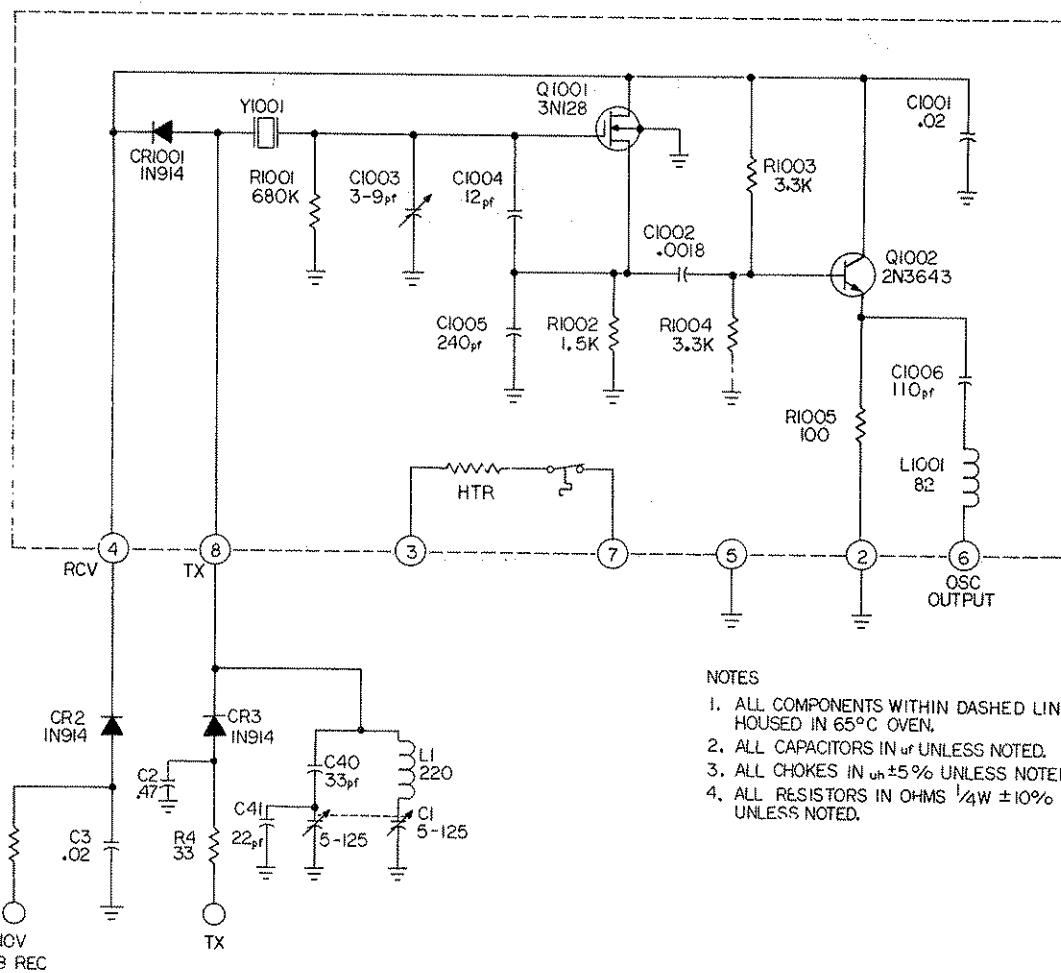
Figure X-20 1- P.C. #10, 1650 OSCILLATOR
