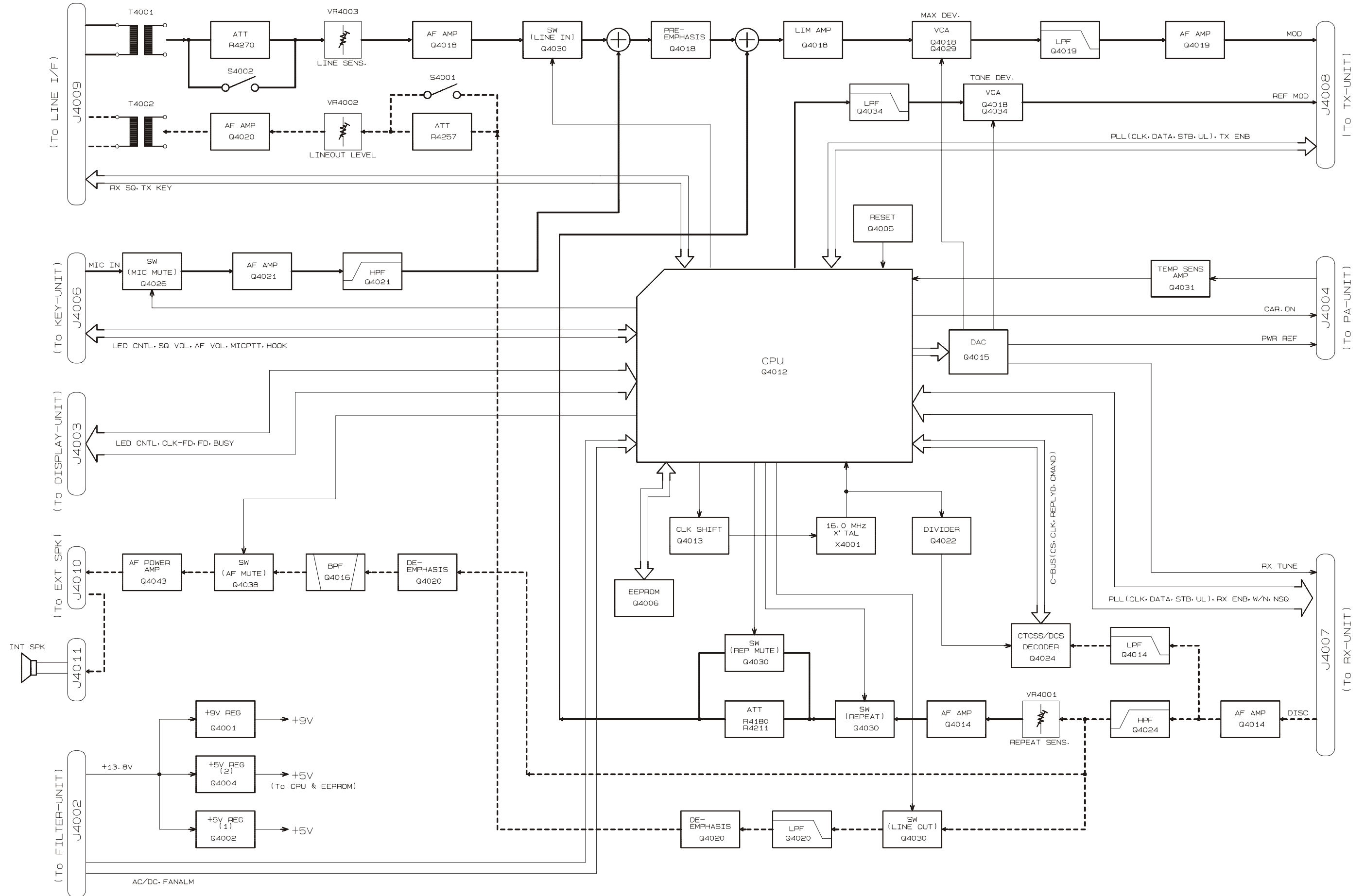
CNTL BLOCK-DIAGRAM
