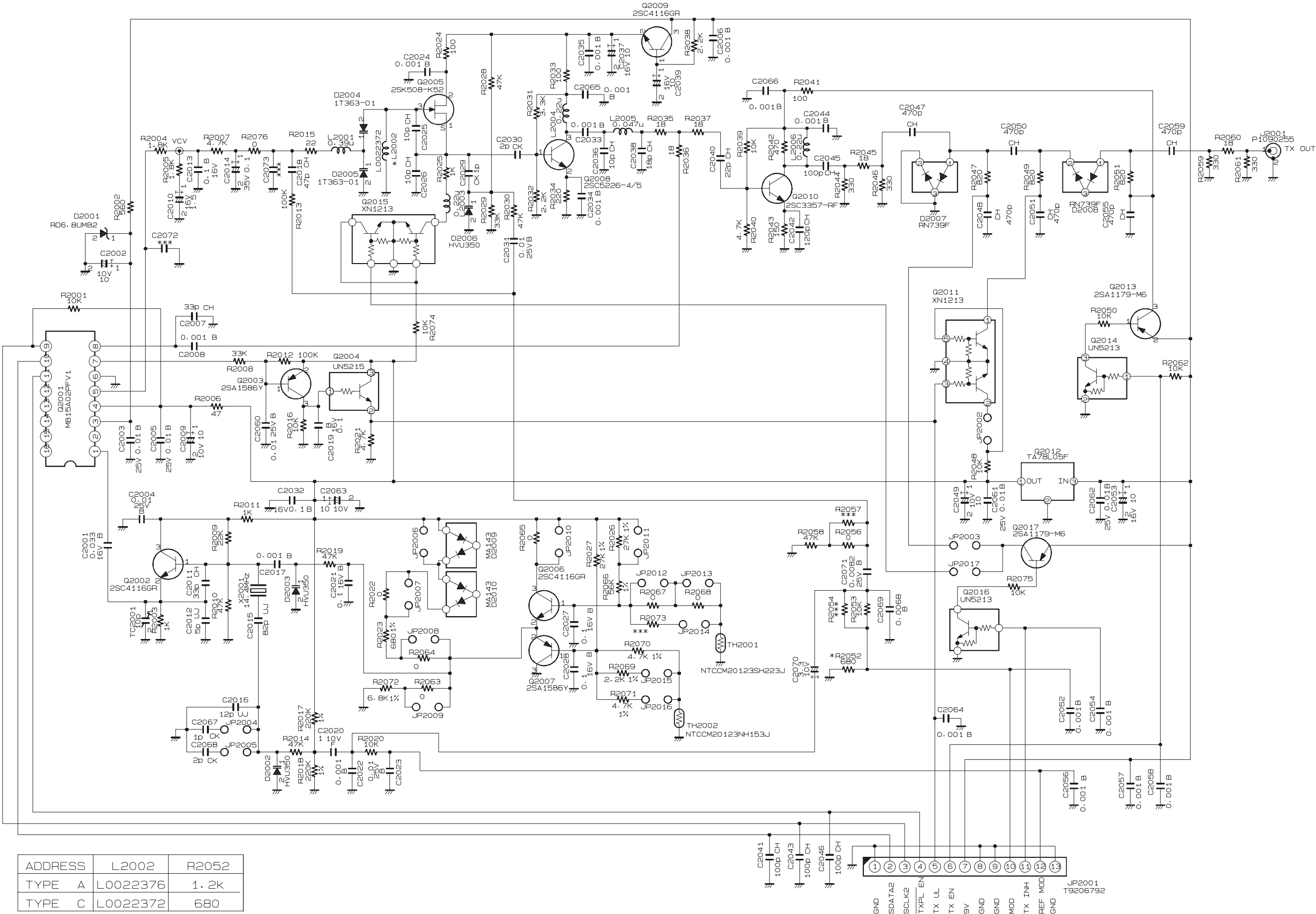
Circuit Diagram
