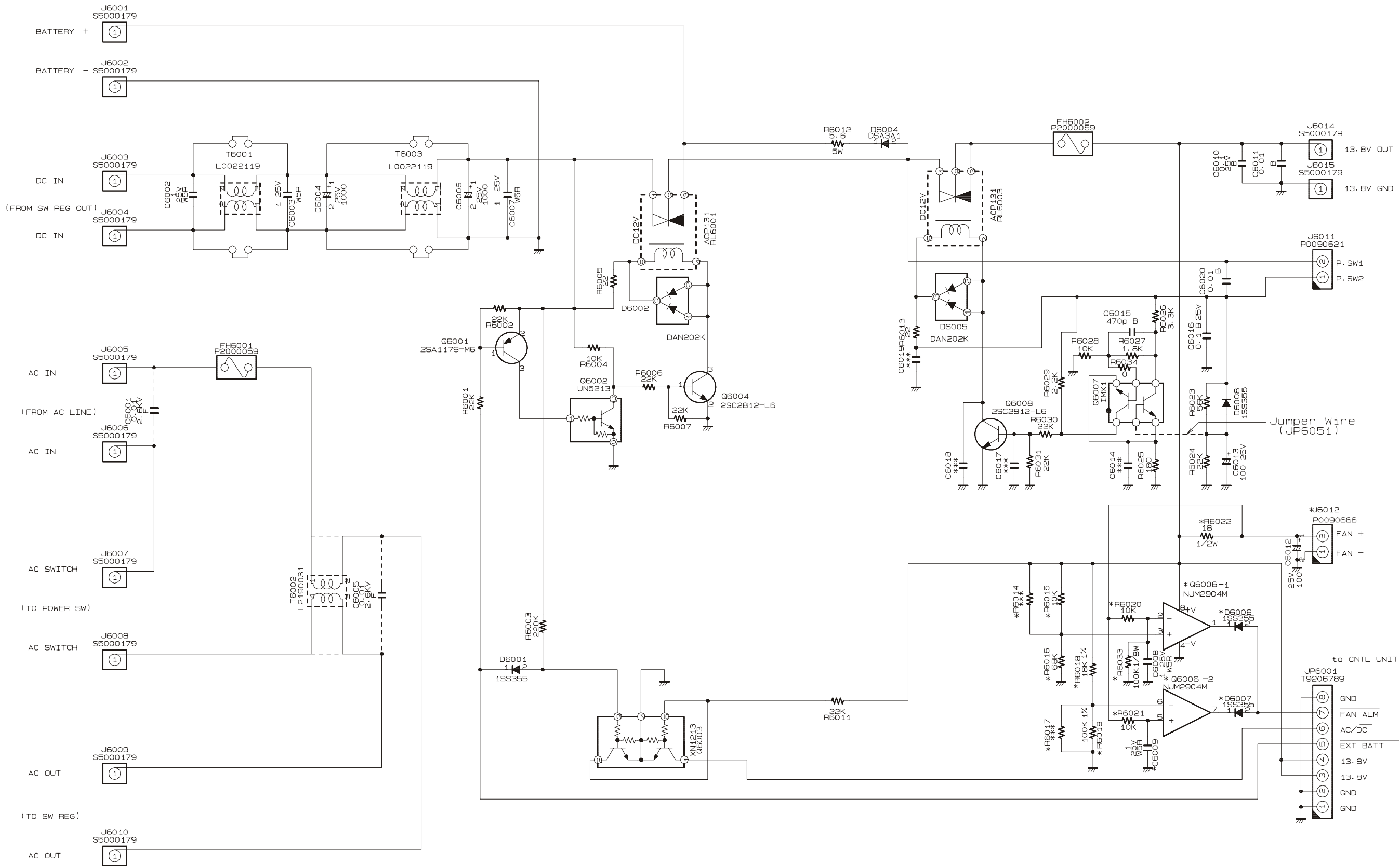
Circuit Diagram
