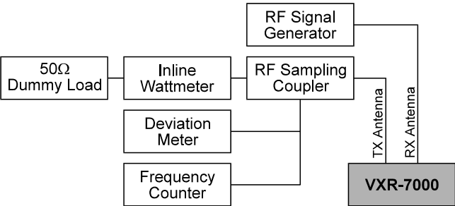
Alignment Setup
